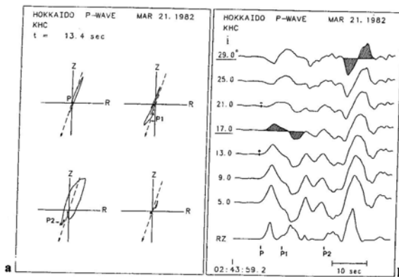
Fig. 2. a Particle motion diagrams in the R-Z (radial-vertical) plane for a=41^\circ . The dashed line indicates the theoretical incidence angle, i_0=17^\circ . b v'_L - v'_Q traces for the determination of the average apparent incidence angle i for the P wave group shown in Fig. 1 using the condition \int [v'_L(a, i) - v'_Q(a, i)] dt = 0 . Integration intervals and labels as in Fig. 1b. The first-motion and average apparent incidence angles are in the same interval, [15^\circ, 19^\circ]
