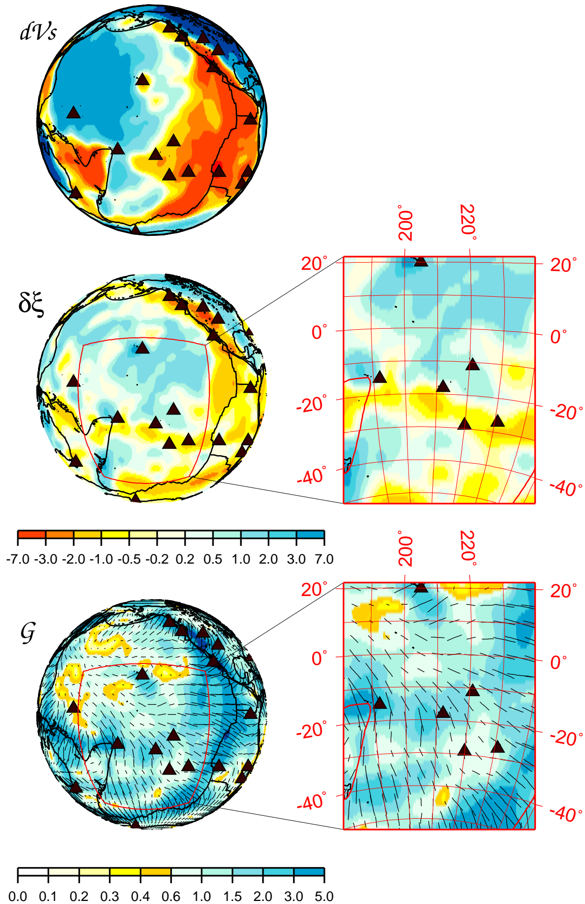
Figure 2a,b Azimuthal, Radial Anisotropy and V_S
