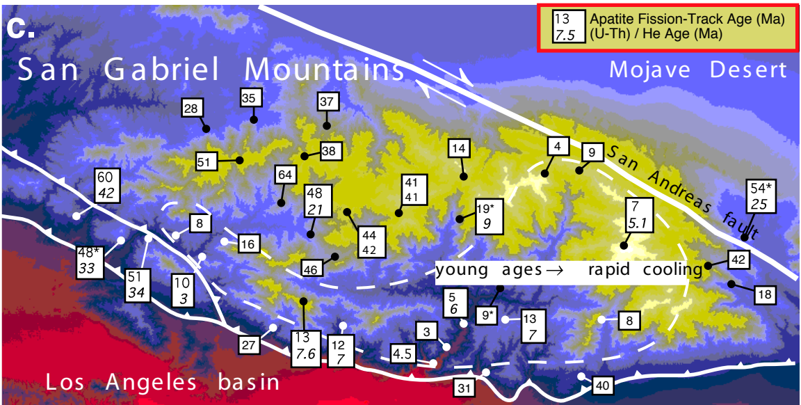
Figure 10.28: Transpressional deformation in the Big Bend, California.
