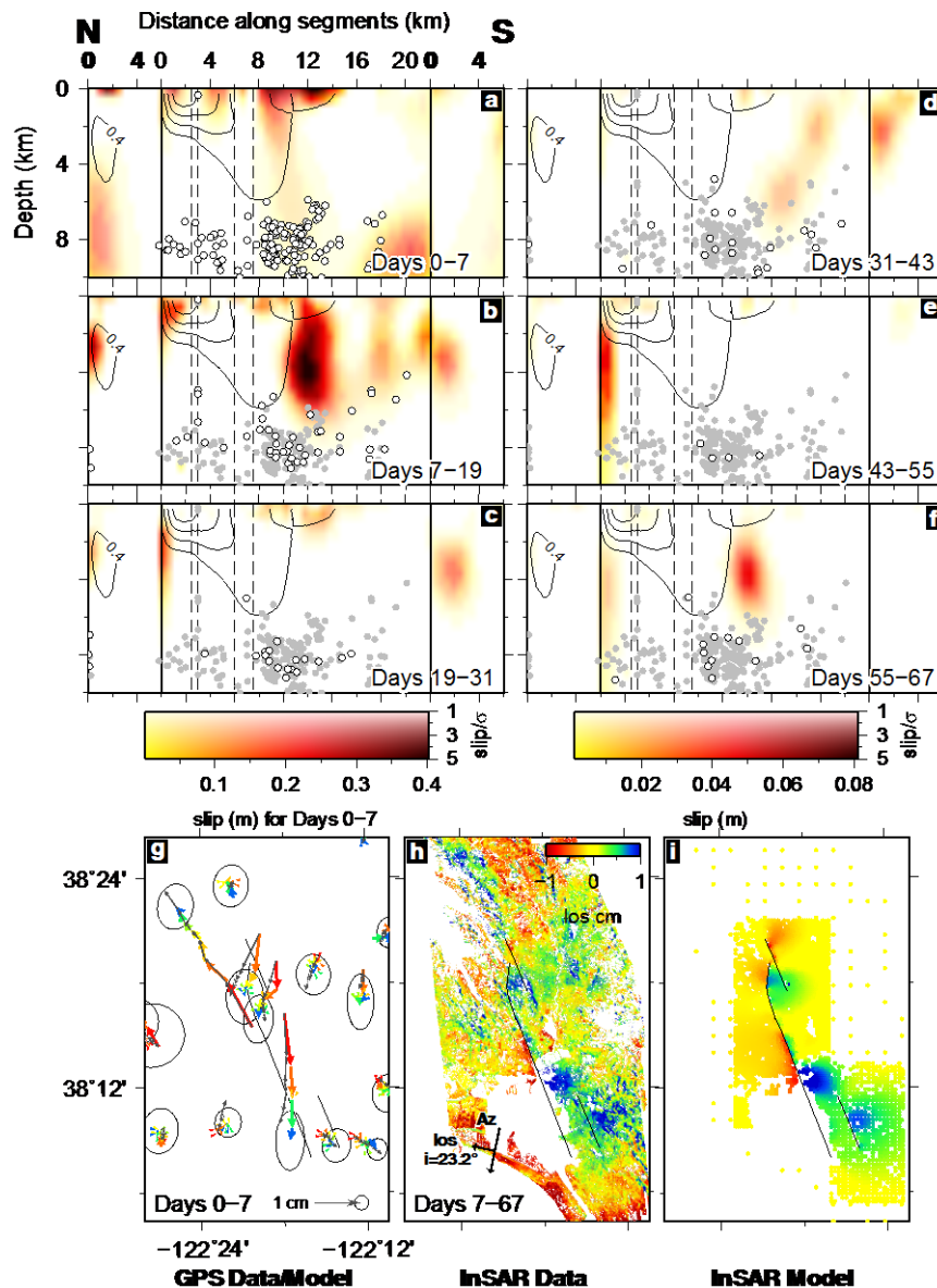
Figure 2. Fault afterslip distributions, and cumulative geodetic data and model. a, b, c, d, e, f Incremental slip distributions on the model fault plane over the annotated intervals. Higher confidence (ratio of slip magnitude-to-uncertainty) estimates are represented by darker color saturations. Black contour lines on each panel represent the coseismic slip shown in Figure 1c, whilst the dots show aftershock locations, projected orthogonally onto the fault plane, during (white) and before (gray) the current time interval. Solid vertical lines delineate the step-over segment (north), main segment (center) and Napa airport segment (south), and dashed vertical lines represent changes in strike on the main segment, as in Figure 1c. g Cumulative GPS displacements for the first seven days following the earthquake are shown by colored vectors (red for displacement on day 1 through to blue for displacement on day 7 after the earthquake), with ellipses showing one-sigma uncertainties on the cumulative displacement. Gray arrows show the model fit to the data. h, i Cumulative InSAR line-of-sight displacement data for days 7–67 following the earthquake ( h ), and modeled displacements displayed for downsampled data points only (see Section 2.1) ( i ). The black lines show the surface trace of the model fault.
