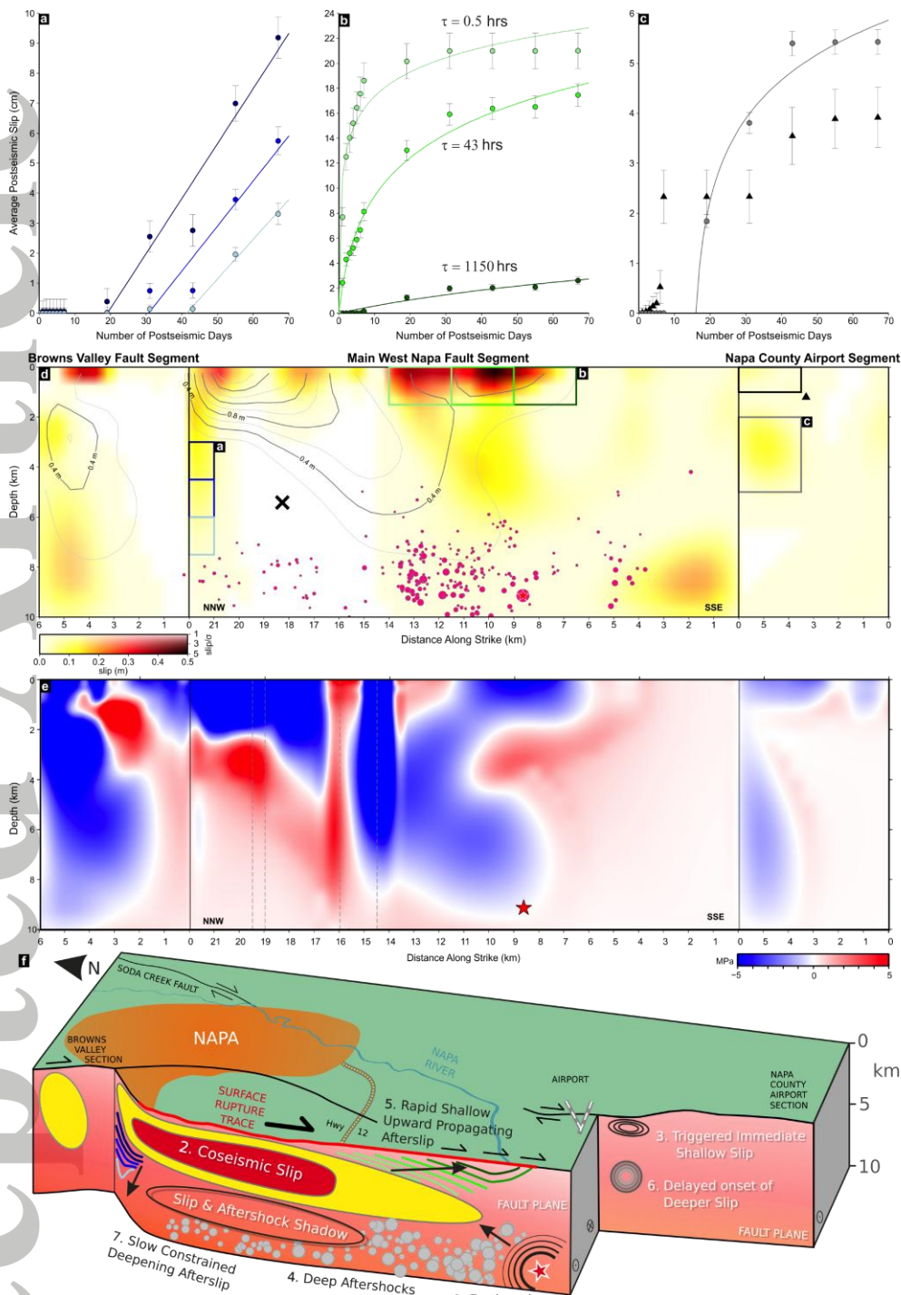
Figure 3. Variable behavior in time and space of afterslip, and relationship of cumulative slip to coseismic Coulomb stress changes and aftershocks. a, b, c Temporal evolution of characteristic slip on patches of the fault. d Cumulative slip distribution across the model fault plane, where colored boxes correspond to the patches shown in the slip evolution time series, above. Segmentation of the model fault is as in Figures 1c and 2. e Coulomb stress change on the West Napa Fault plane due to modeled coseismic slip distribution (see Figure 1c). f Schematic summary of our findings, as described in the text, showing the sequence of slip behavior.
