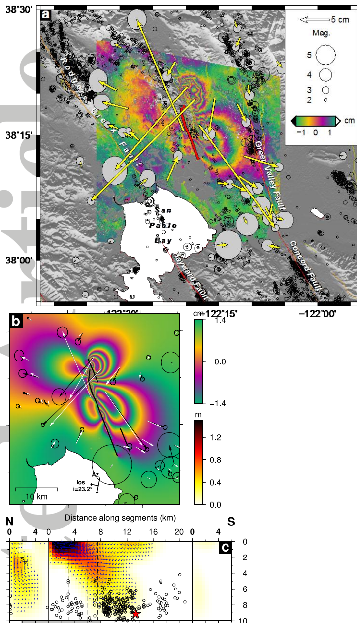
Figure 1. Summary of coseismic geodetic data and model for the 2014-08-24 South Napa earthquake. a Tectonic map of the epicentral region showing pre-earthquake seismicity [Waldhauser, 2009] (black circles), mapped surface rupture of the South Napa earthquake [Morelan et al., 2015] (thick red line), horizontal coseismic GPS displacements (yellow vectors) with 95% confidence ellipses, and line-of-sight InSAR displacements (color map); b Result of data inversion showing the model faults used (black lines), GPS displacement data (black vectors), predicted GPS displacements (white vectors) and predicted InSAR; c View of the modeled coseismic slip on the fault plane. Solid vertical lines delineate the separate (from left to right) northern step-over segment, main segment and southeastern Napa airport segment; dashed vertical lines represent changes in strike along the main segment, as shown in (b). The hypocenter is marked by the red star and aftershocks by black circles. Contours of coseismic slip are at 0.4 m intervals.
