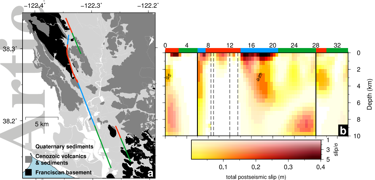
Figure 4. Spatial relationship between the major types of lithological units and the co- and post-seismic slip patterns during the 2014 earthquake. a Along-strike variations of slip type, shown as fault segments colored red (predominant coseismic slip or triggered slip), blue (major afterslip), or green (minor or insignificant coseismic or postseismic slip). The background, adapted from the geological map of Napa County from Graymer et al. [2006, 2007] and references therein, shows the distribution of the major geologic units: black represents Cretaceous basement rocks from the Franciscan Complex, mostly the Great Valley Sequence; dark gray represents consolidated Cenozoic volcanic and sedimentary rocks, including Sonoma Volcanics; light gray represents Quaternary alluvial deposits. b Corresponding slip, as modeled in this study. Color shows total afterslip to day 67, contours show coseismic slip. Panel is the same as in Figures 1c, 2a-f and 3b. Red, blue and green lines demarcate the same along-strike variations as described for (a).
