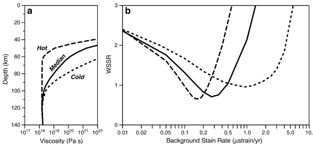
Fig. 5. (a) Calculated viscosity based on dislocation creep of wet olivine (median parameters, Table 1), a differential stress of 0.3 MPa, water content of 800 H/10 6 Si, and the three thermal gradients shown in Figure 3a. (b) Misfit of calculated cumulative (7 years) postseismic surface displacements as a function of background strain rate and thermal gradient.
