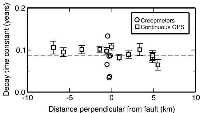
Figure 5. Decay time constants fit to continuous GPS data (squares) and creepmeter data (circles). Dashed line shows average value (0.087 years) used in time-series and slip modeling. Uncertainties for the creepmeter data average 0.003 years; error bars would be about the size of the symbol ( \text{\textcircled{E}} Table S3 in the electronic edition of BSSA).
