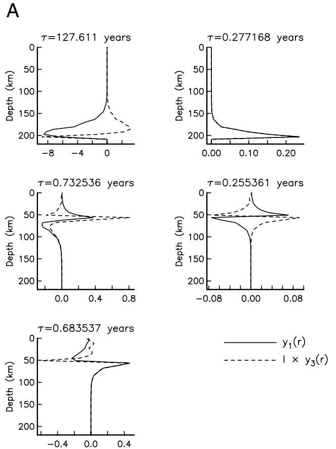
Figure 4. Mode eigenfunctions y_1(r, s_j) and l \times y_3(r, s_j) normalized by \sqrt{\epsilon_j s_j} on rheology 1. (a) Stable relaxation modes of l = 545 for 1/s_j < 3.189 \times 10^5 yr. (b) Stable relaxation modes of l = 545 for a few modes with 1/s_j > 3.189 \times 10^5 yr. (c) Unstable (RT) relaxation modes of l = 545 for the five fastest growing modes.
