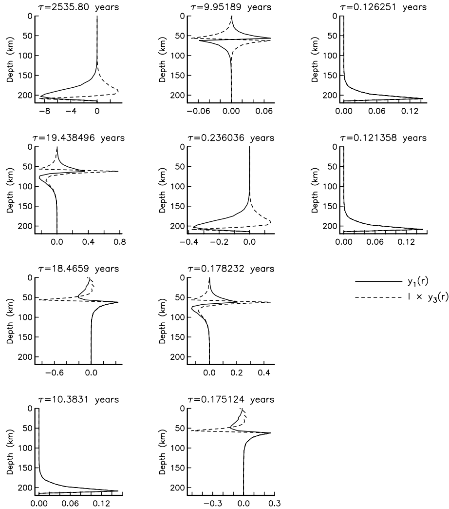
Figure 7. Mode eigenfunctions y_1(r, s_j) and l \times y_3(r, s_j) normalized by \sqrt{\epsilon_j s_j} on rheology 2. Stable relaxation modes of l = 545 for 1/s_j < 3.189 \times 10^5 yr.
