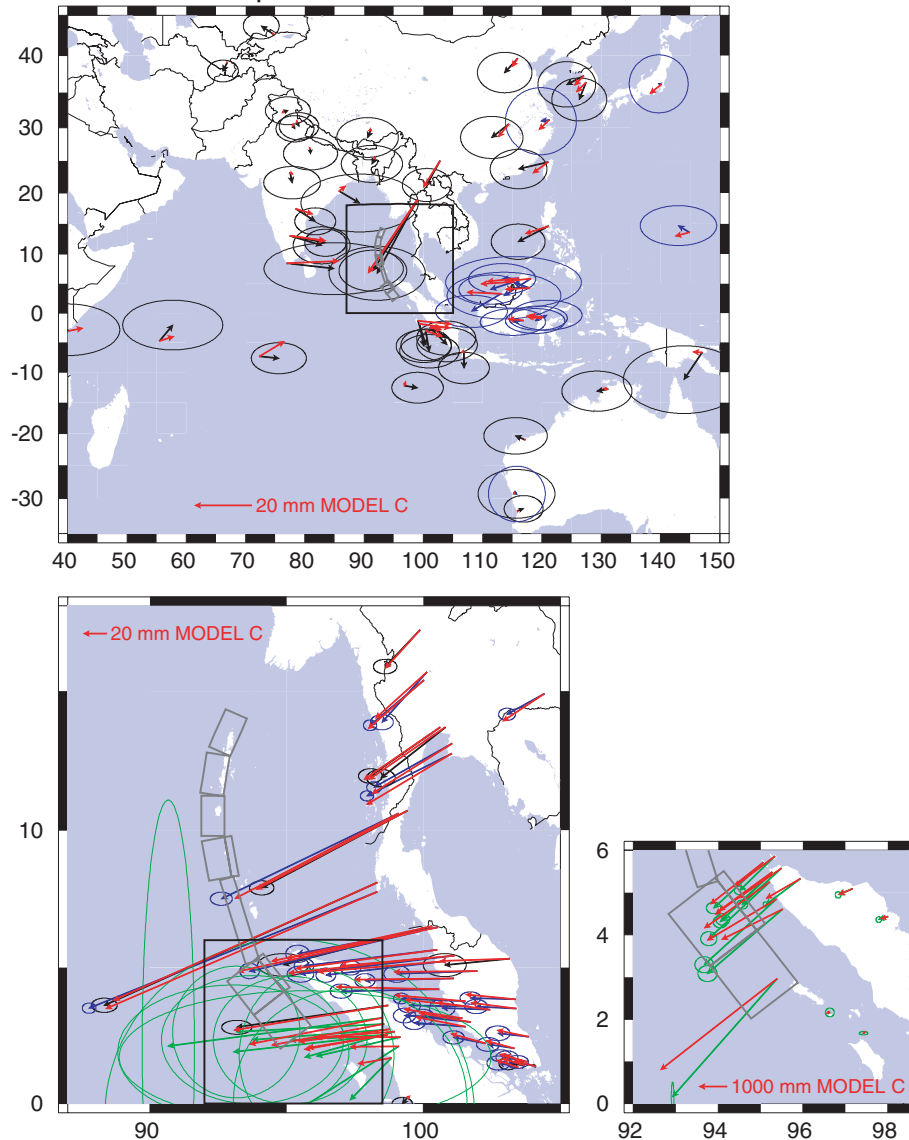
Figure 8. Coseismic horizontal displacement field of the 2004 December 26 earthquake shown by black vectors with 95 per cent error ellipses, together with the ‘corrected’ coseismic offsets derived from Tables 1 and 2 of Vigny et al. (2005), shown by the blue vectors, and coseismic offsets derived from campaign GPS from Table S1 of (Subarya et al. 2006), shown by the green vectors. Superimposed red vectors are the predicted static displacements on the PREM model using slip Model C of Banerjee et al. (2006). Grey lines indicate the fault planes used to obtain Model C.
