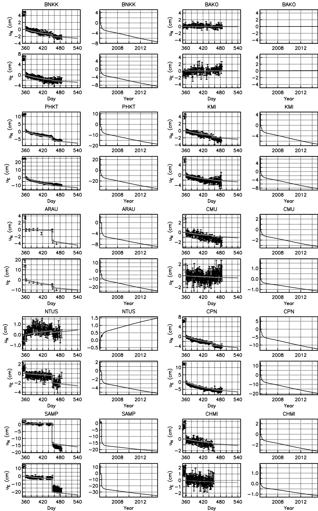
Figure 13. Same comparison as in Fig. 12, but with model time-series calculated on rheology 2.
