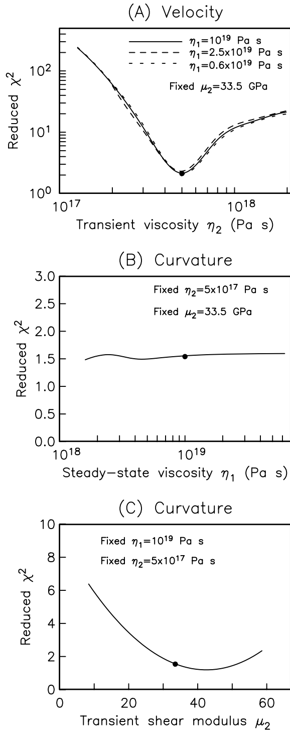
Figure 16. (a) \chi_v^2 and (b and c) \chi_\zeta^2 resulting from viscoelastic models with various combinations of \eta_1 , \eta_2 , and \mu_2 . Note that there is little sensitivity of either v or \zeta to \eta_1 . Filled circles indicate the fit of rheology model 2.
