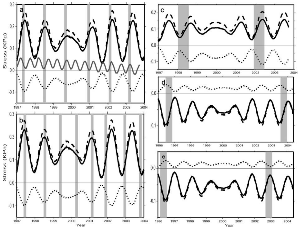
Figure 2. Pole-tide-induced stress-change time series. Solid curve is the Coulomb failure stress change on the slab interface, dashed and dotted curves are its shear and normal components, respectively. Fault normal tension and thrust-sense shear stress are positive. Gray vertical stripes are the epochs of the ESS events. (a) northern Cascadia, (b) southern Cascadia, (c) Guerrero, (d) Bungo Channel, and (e) Boso Peninsula subduction zones. Gray curve in (a) is the Coulomb failure stress change induced by annual and semiannual Earth tides.
