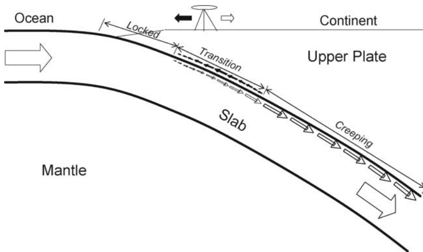
Figure 1. Schematic view of tectonic setting of subduction zone and occurrence of ESS events. Large open arrows mark the secular motion of the oceanic plate relative to the continental plate, with the relative motion across the plate interface shown by open arrows. The small open arrow next to the GPS antenna points to its secular motion direction with regard to the interior of the continental plate. Solid arrows on the plate interface show the episodic slow slip events that occurred in the locked-to-creeping transition zone, with their associated surface motion direction indicated by a solid arrow next to the GPS antenna.
