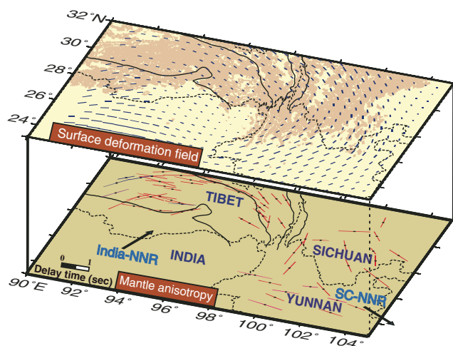
Figure 3. Three-dimensional block diagram: top is surface deformation field plotted as left-lateral shear directions (in blue) and bottom is slice through upper-mantle layer displaying seismic anisotropy. Surface layer includes global positioning system-derived left-lateral shear strain, geological sutures, and province boundaries. Elevations above 5000 m are embedded in background in light brown. Mantle layer includes splitting measurements from our study, and vectors displaying absolute plate motion of Indian plate and of South China block (SC) calculated using ITRF2000-No-Net-Rotation (NNR) frame (Altimimi et al., 2002). Figure shows similar pattern between surface strain field and mantle anisotropy wrapping around eastern Himalayan syntaxis. Sharp transition in splitting pattern is observed when moving south away from Plateau at ~lat 26°N. Province boundaries are plotted as black dotted lines.
