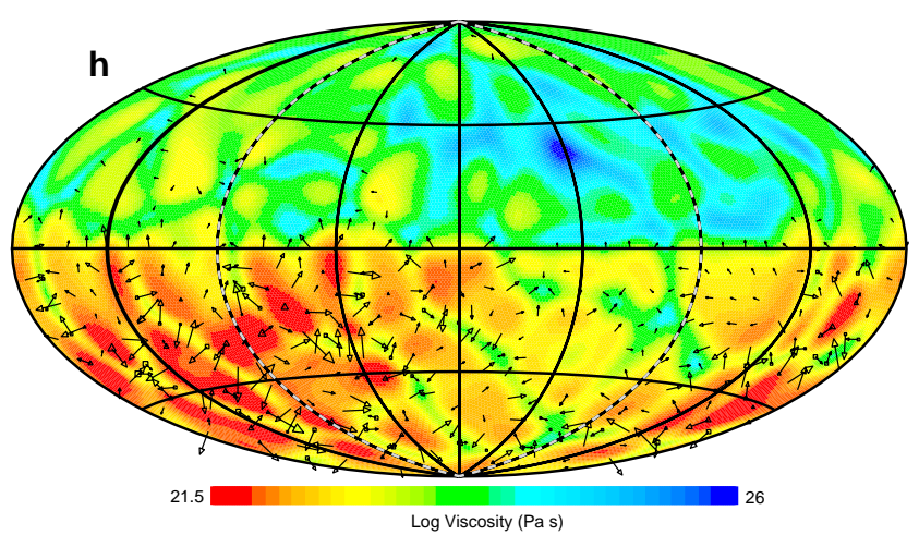
Hemispheric Dichotomy Model
