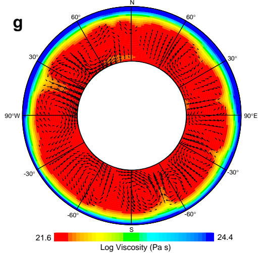
Log Viscosity (Pa s)
