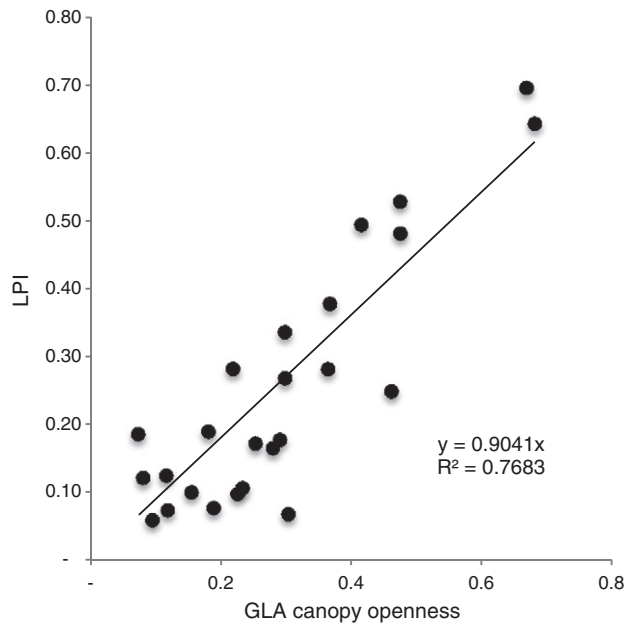
Fig. 12. LPI vs. GLA canopy openness.
