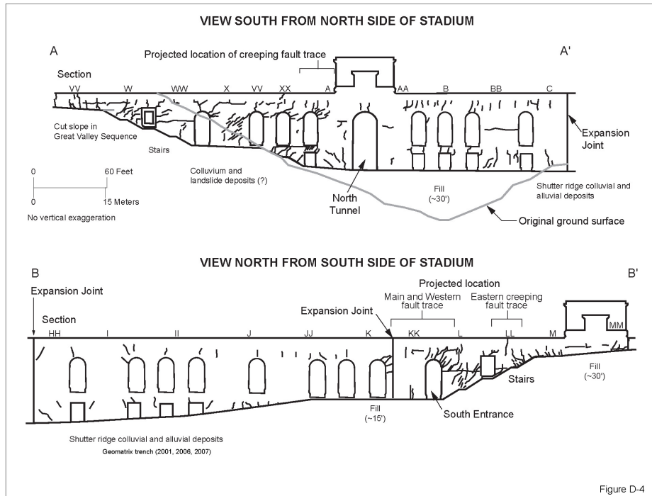
Figure D-4: Elevation views of the northern (A) and southern (B) sides of Memorial Stadium. Diagonal, vertical, and horizontal fractures are interpreted as fault related, settlement induced, and construction induced, respectively.
