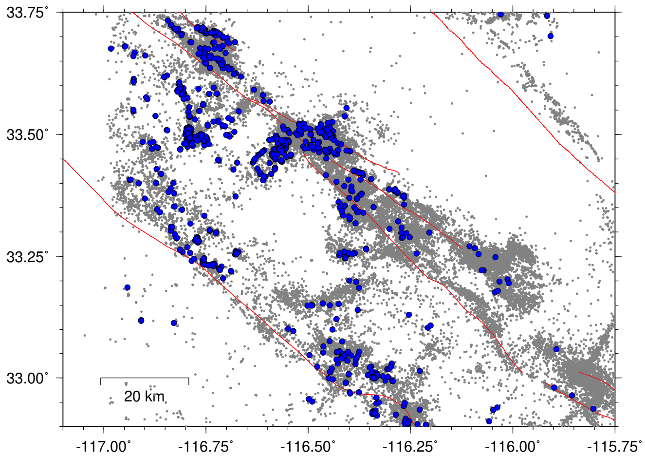
SSAF Repeating earthquakes mincoh \geq 9500 life_span \geq 0days
