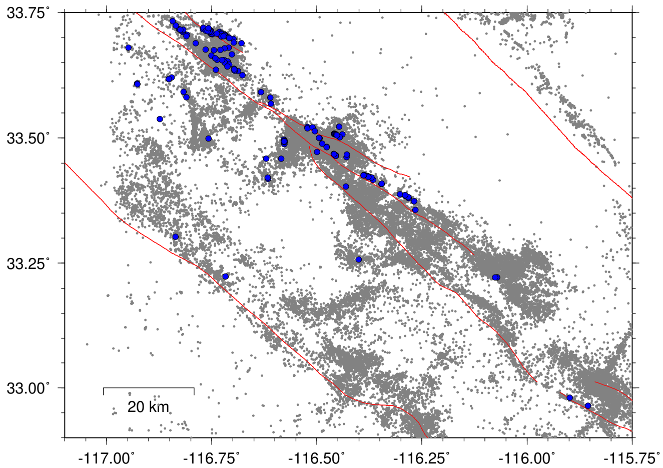
SSAF Repeating earthquakes mincoh \geq 9500 life_span \geq 1000days
