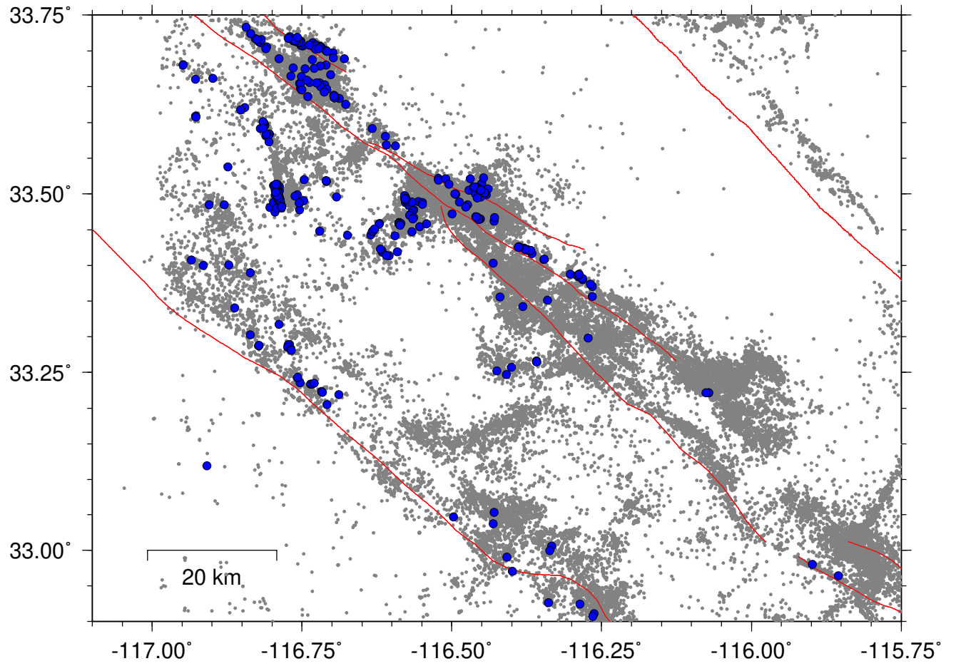
SSAF Repeating earthquakes mincoh \geq 9500 life_span \geq 100days
