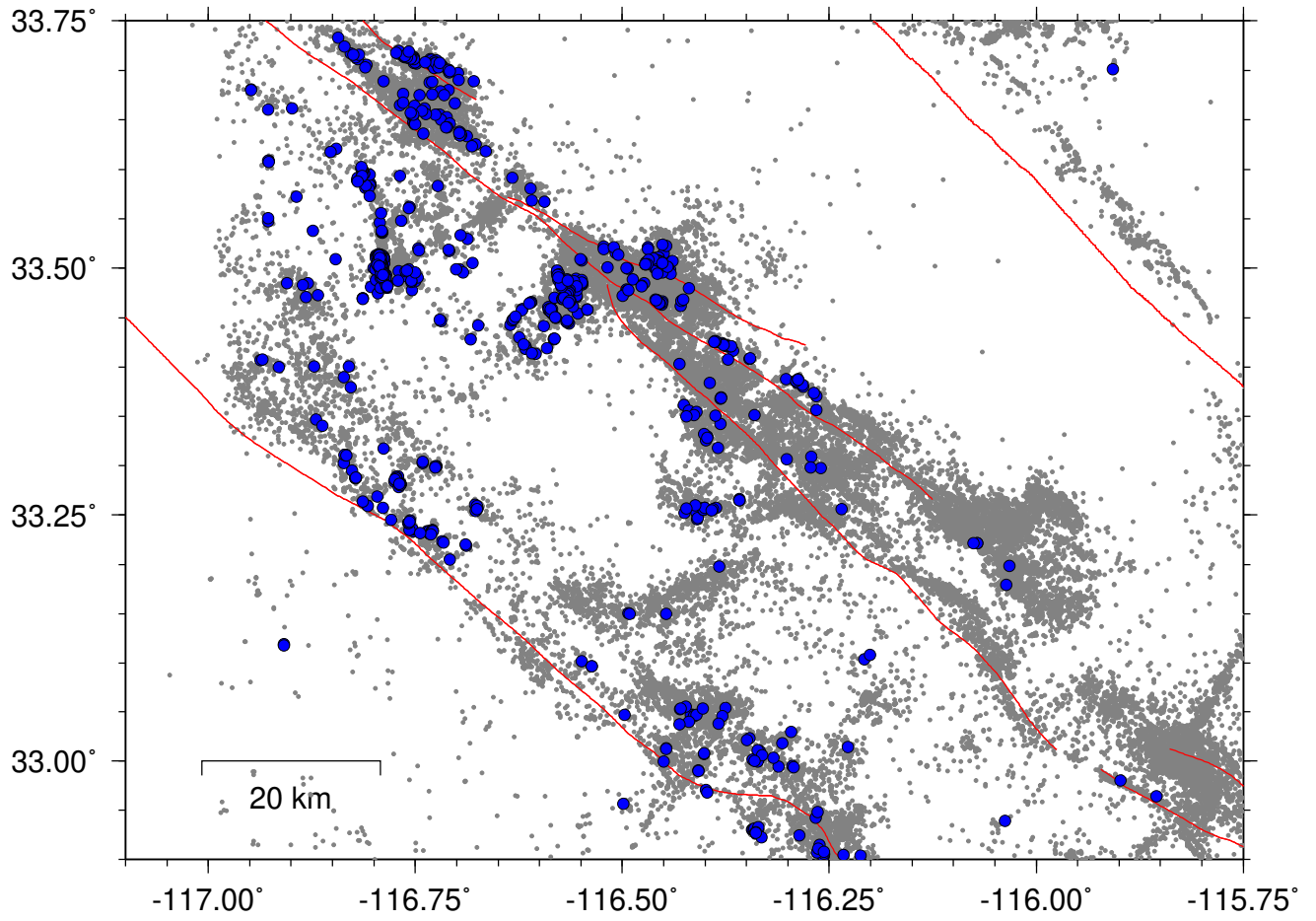
SSAF Repeating earthquakes mincoh \geq 9500 life_span \geq 10days
