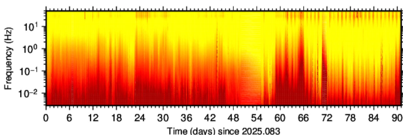
BK.GUMB.HNN.00 (2025.083 - 2025.173)
