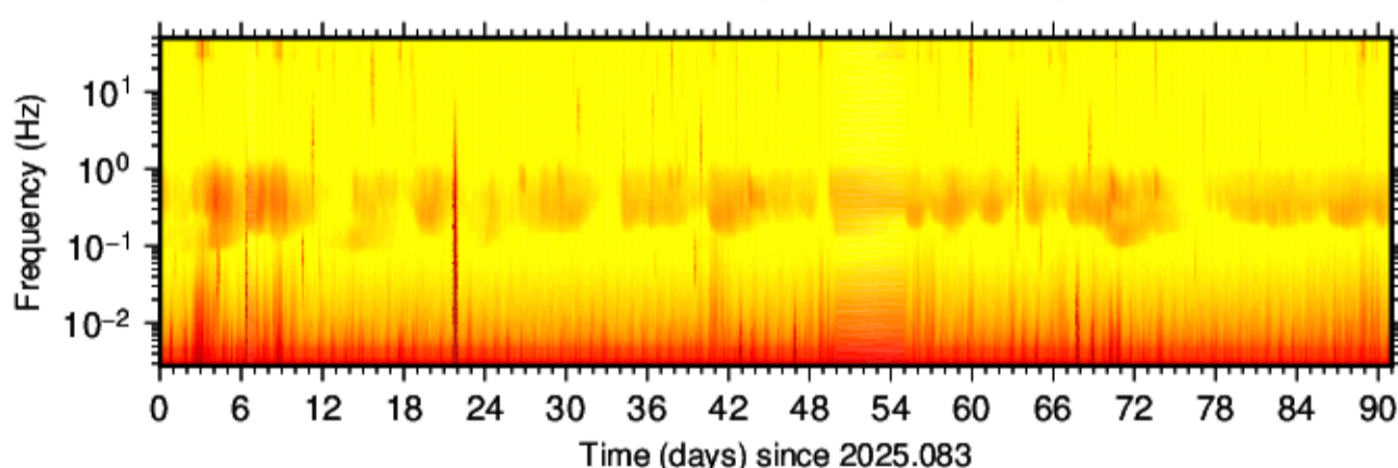
BK.HRCH.HNN.00 (2025.083 - 2025.173)
