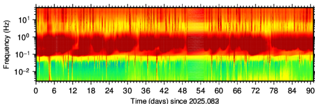
BK.HRCH.HHZ.00 (2025.083 - 2025.173)
