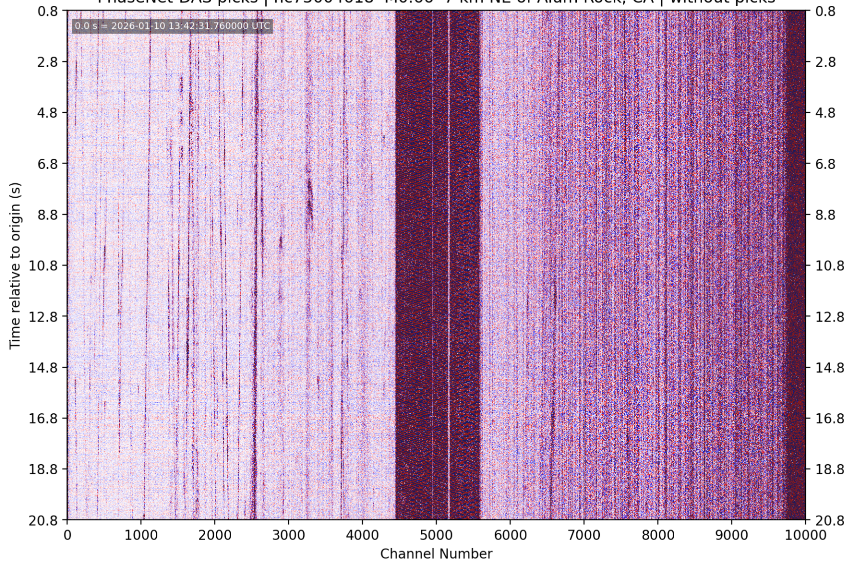
PhaseNet-DAS picks | nc75004618 M0.66 7 km NE of Alum Rock, CA | without picks
