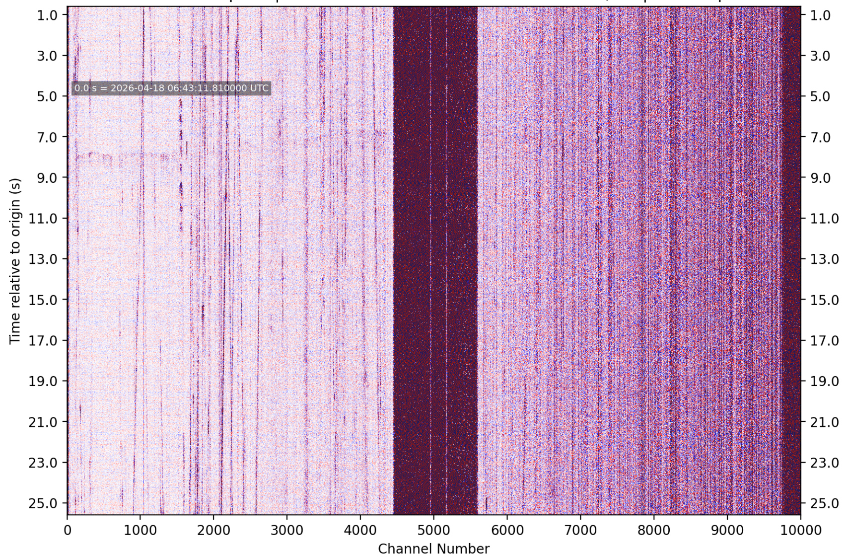
PhaseNet-DAS picks | nc75005153 M1.03 4 km SE of Pacifica, CA | without picks
