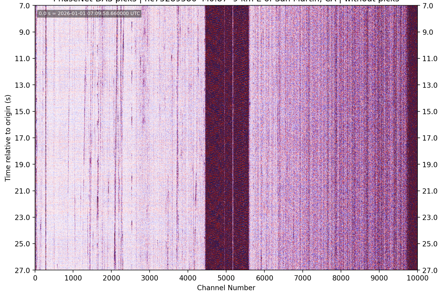
PhaseNet-DAS picks | nc75289586 M0.87 9 km E of San Martin, CA | without picks
