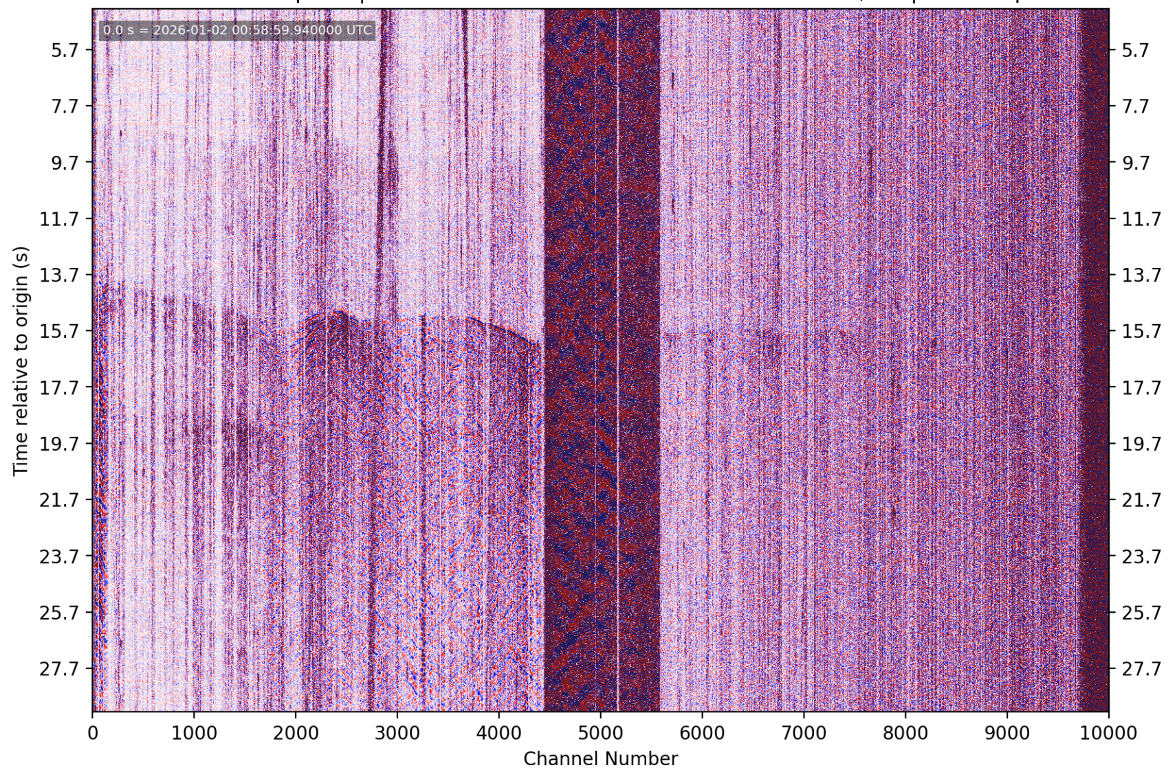
PhaseNet-DAS picks | nc75289861 M3.02 2 km SE of San Ramon, CA | without picks
