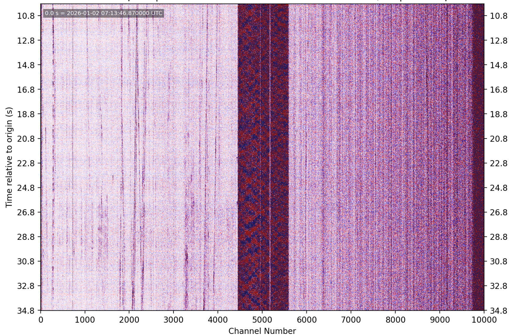
PhaseNet-DAS picks | nc75289911 M2.21 15 km E of Seven Trees, CA | without picks
