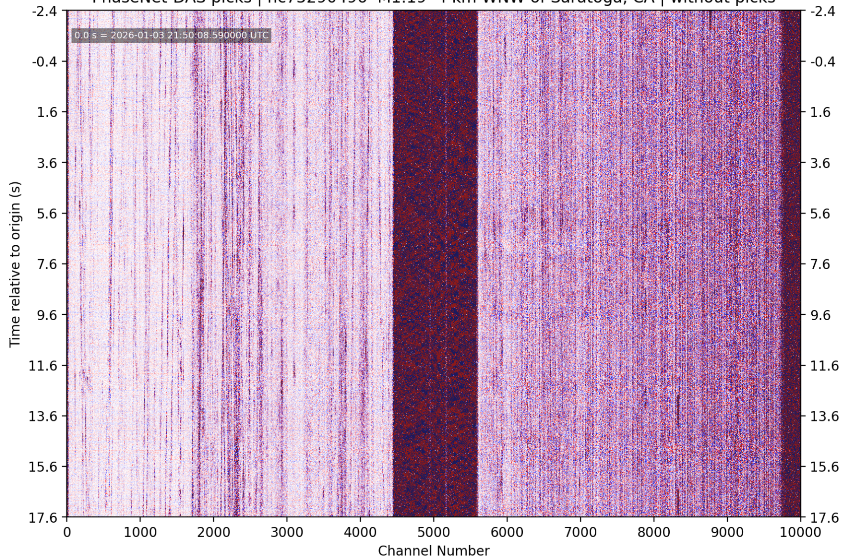
PhaseNet-DAS picks | nc75290496 M1.19 4 km WNW of Saratoga, CA | without picks
