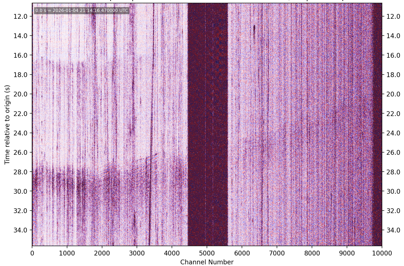
PhaseNet-DAS picks | nc75290936 M2.8 4 km N of Corralitos, CA | without picks
