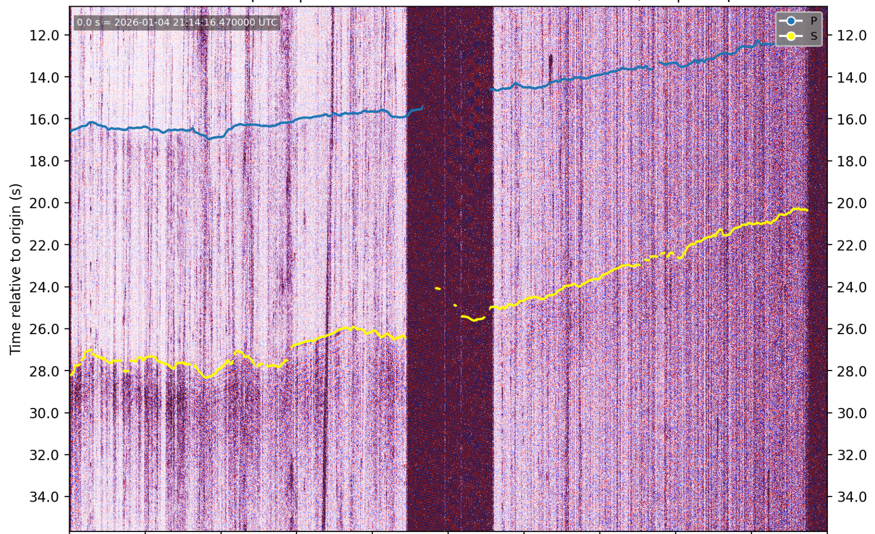
PhaseNet-DAS picks | nc75290936 M2.8 4 km N of Corralitos, CA | without picks
