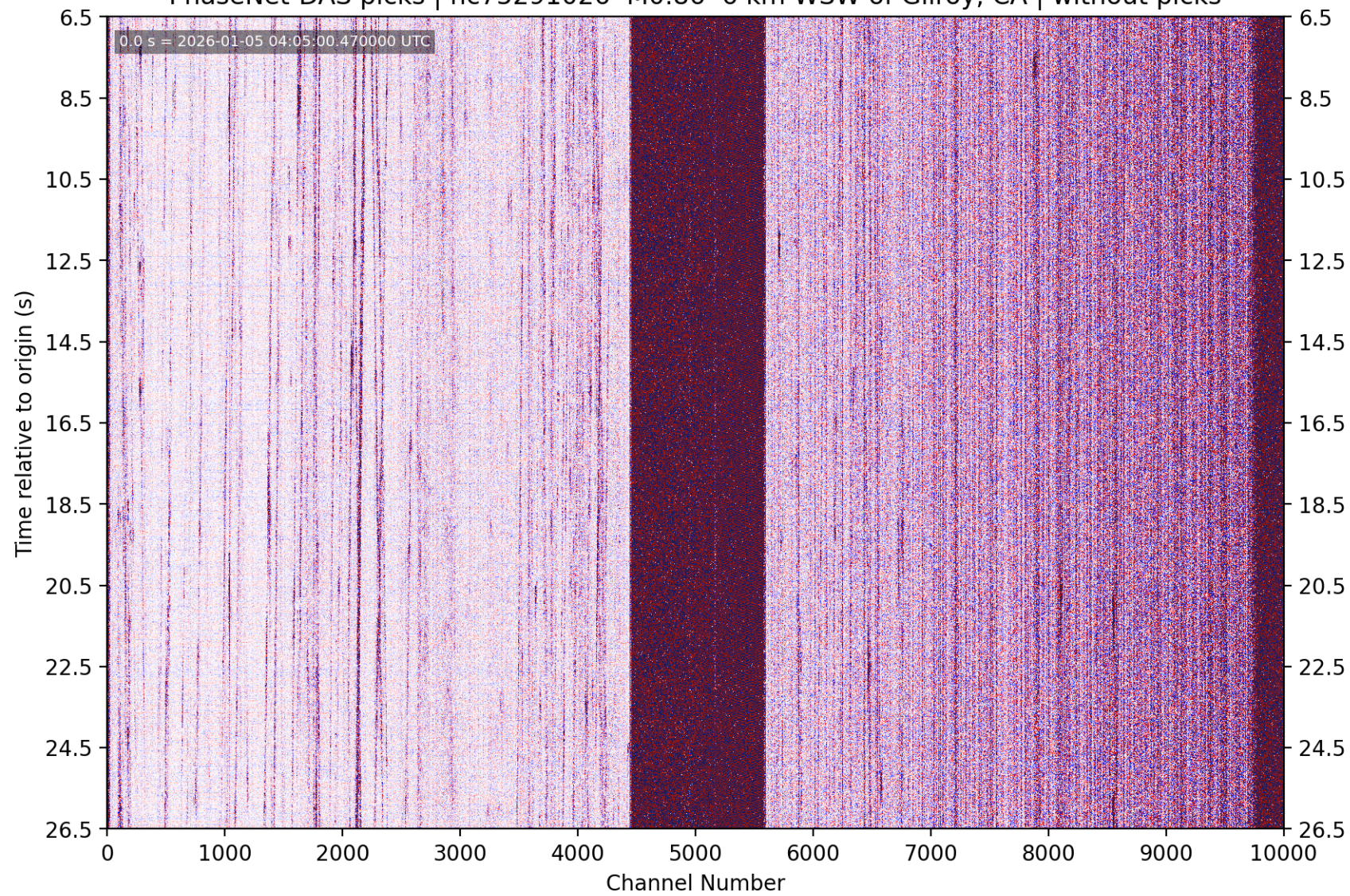
PhaseNet-DAS picks | nc75291026 M0.86 6 km WSW of Gilroy, CA | without picks
