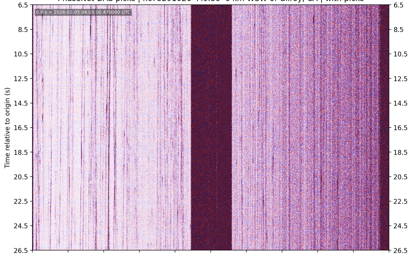
PhaseNet-DAS picks | nc75291026 M0.86 6 km WSW of Gilroy, CA | without picks
