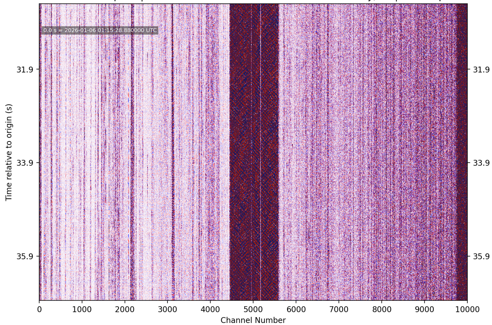
PhaseNet-DAS picks | nc75291361 M1.45 10 km SSE of Portola Valley, CA | without picks
