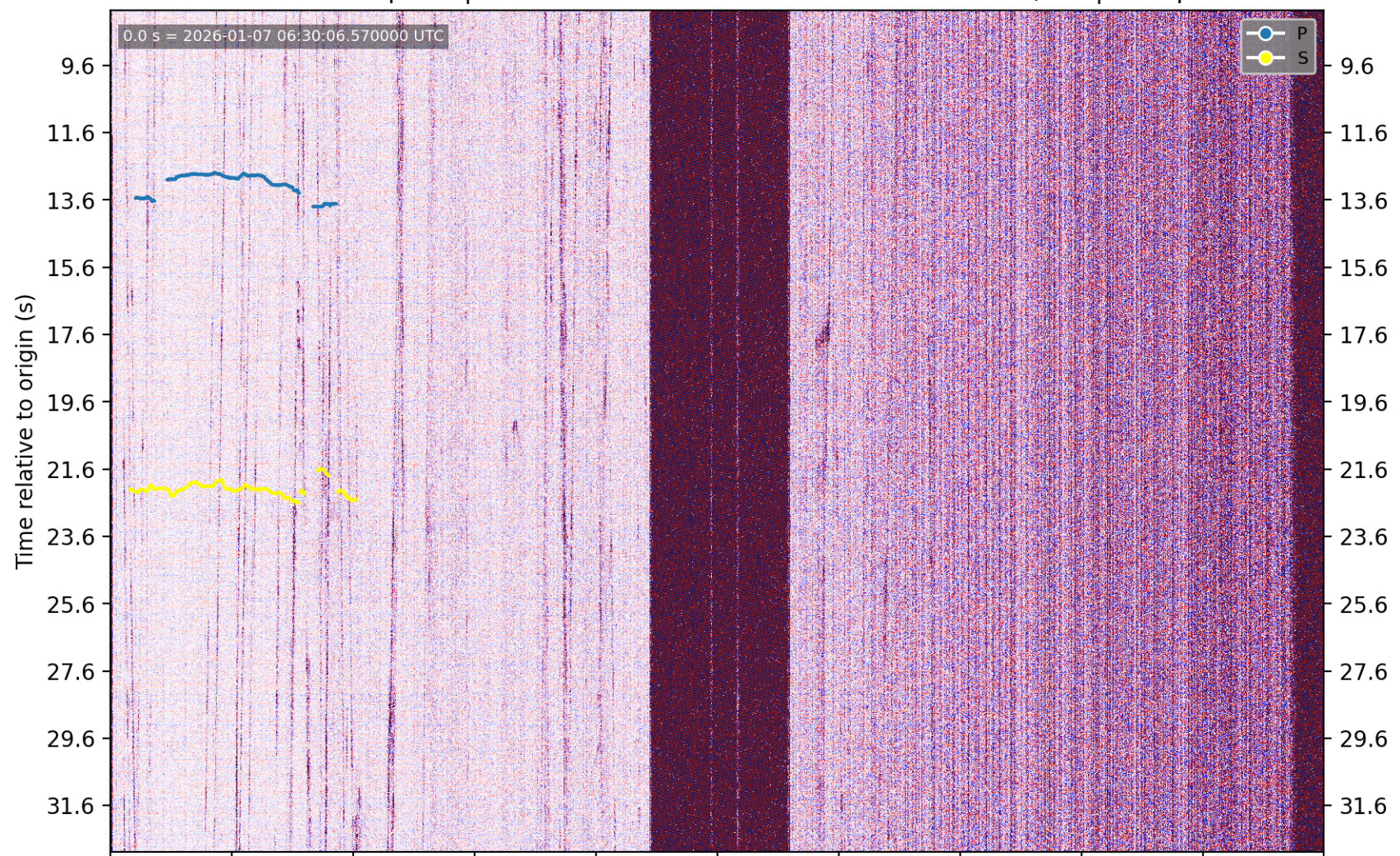
PhaseNet-DAS picks | nc75291901 M1.17 9 km E of Alum Rock, CA | without picks
