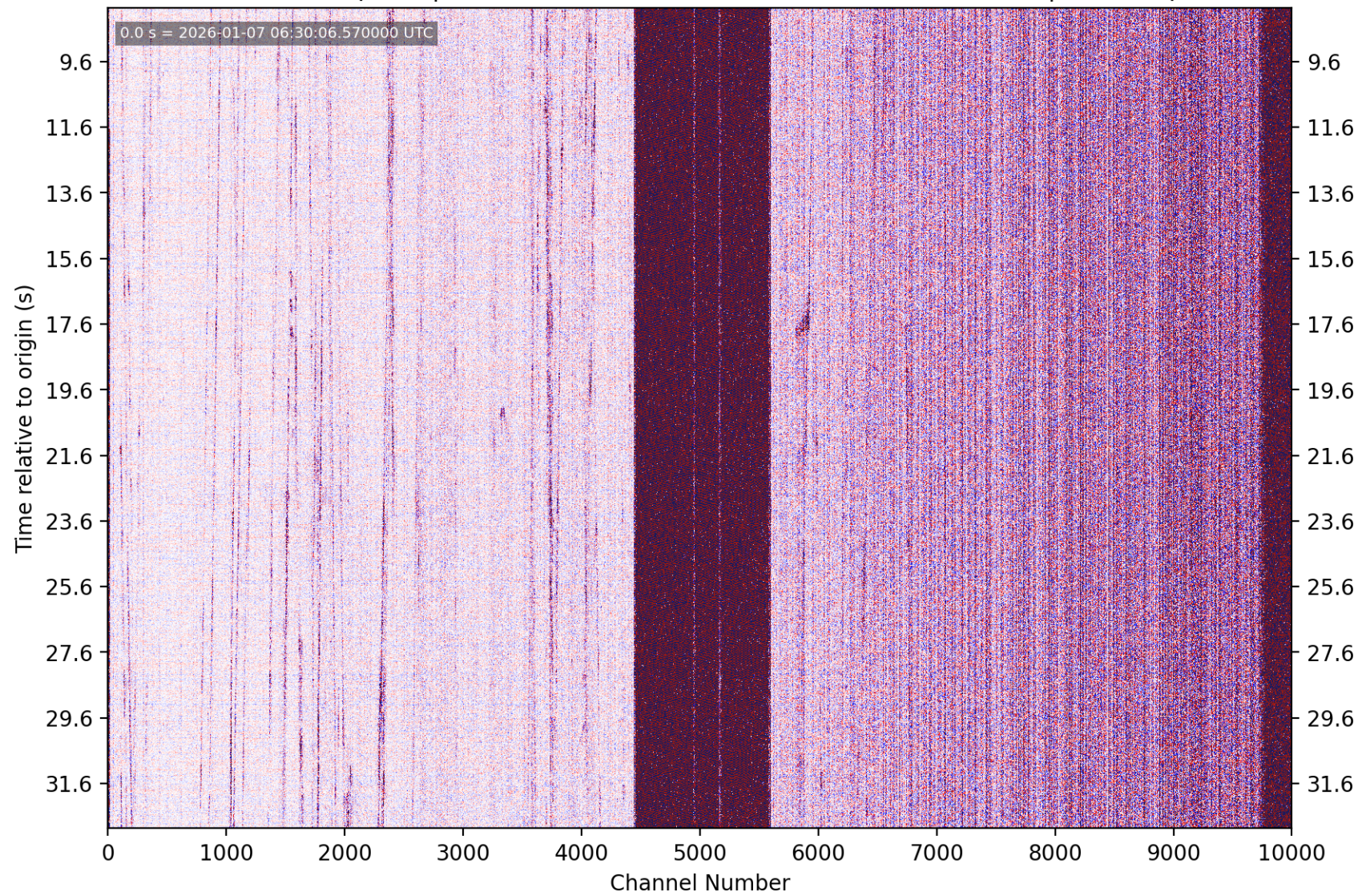
PhaseNet-DAS picks | nc75291901 M1.17 9 km E of Alum Rock, CA | without picks
