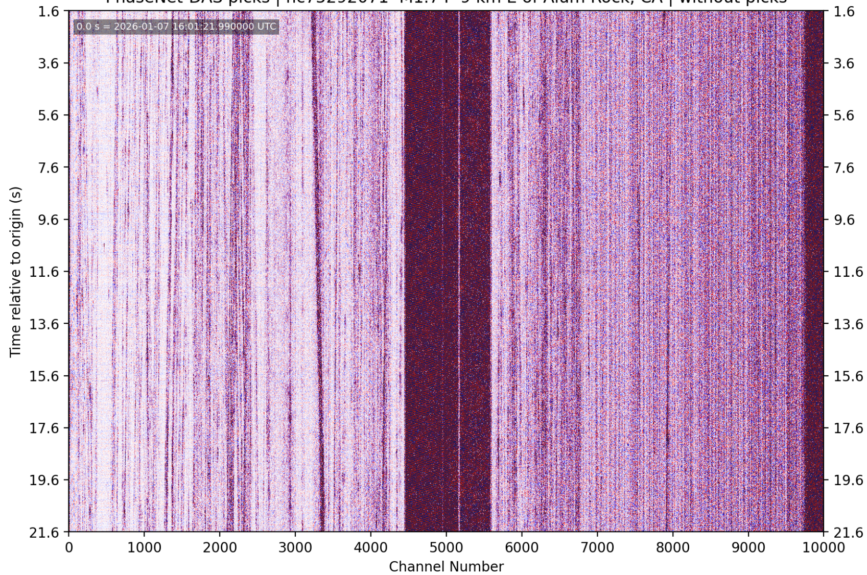
PhaseNet-DAS picks | nc75292071 M1.74 9 km E of Alum Rock, CA | without picks
