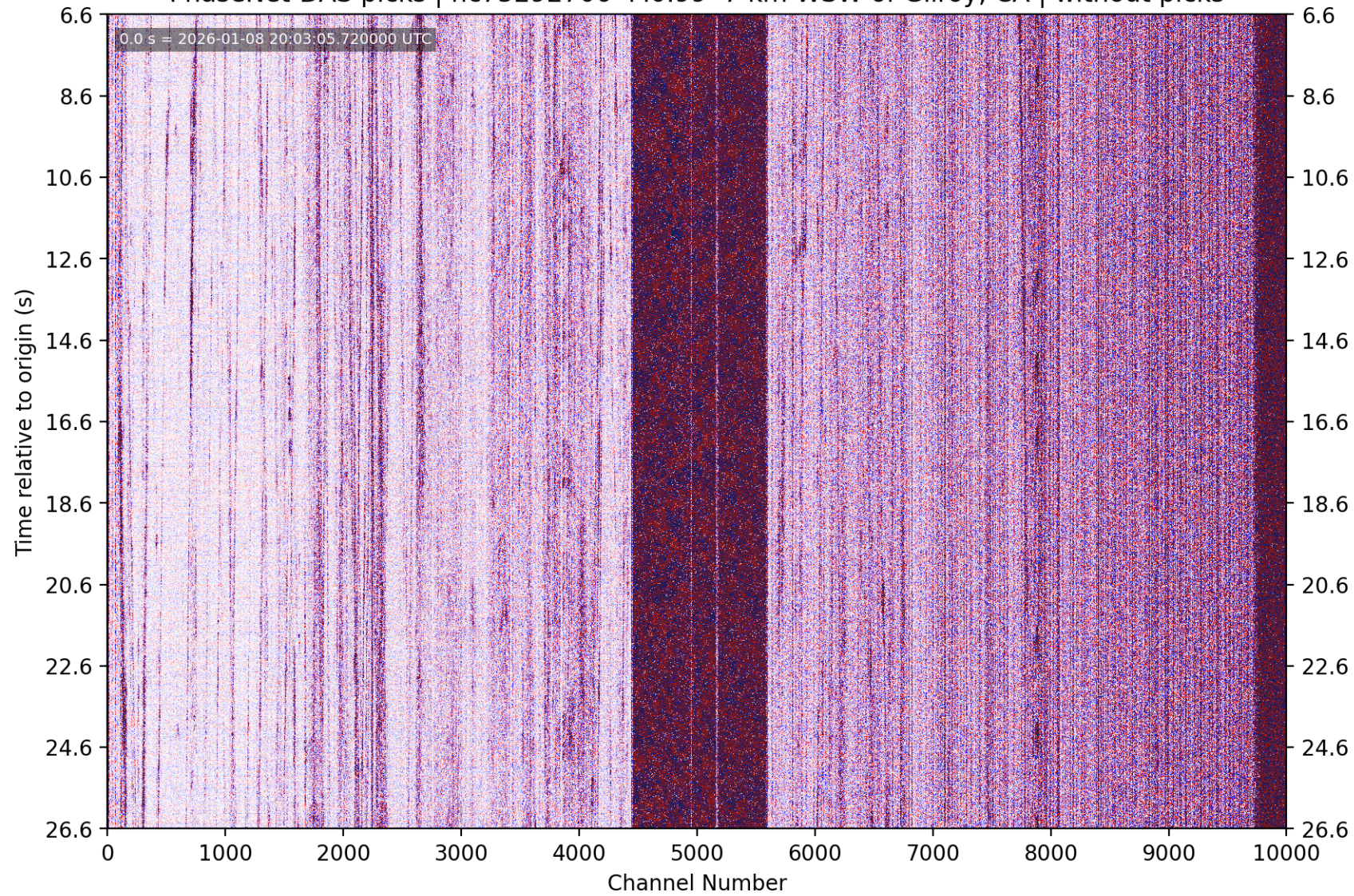
PhaseNet-DAS picks | nc75292706 M0.99 7 km WSW of Gilroy, CA | without picks
