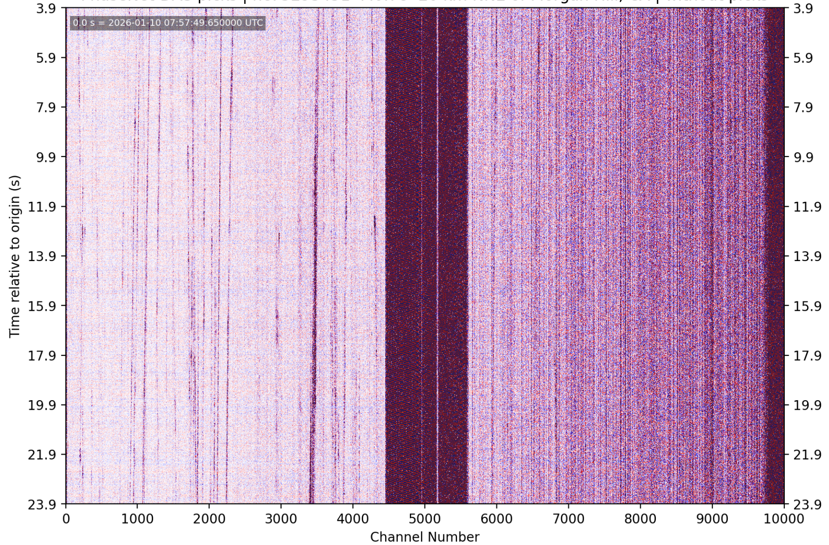
PhaseNet-DAS picks | nc75293451 M0.78 20 km NNE of Morgan Hill, CA | without picks
