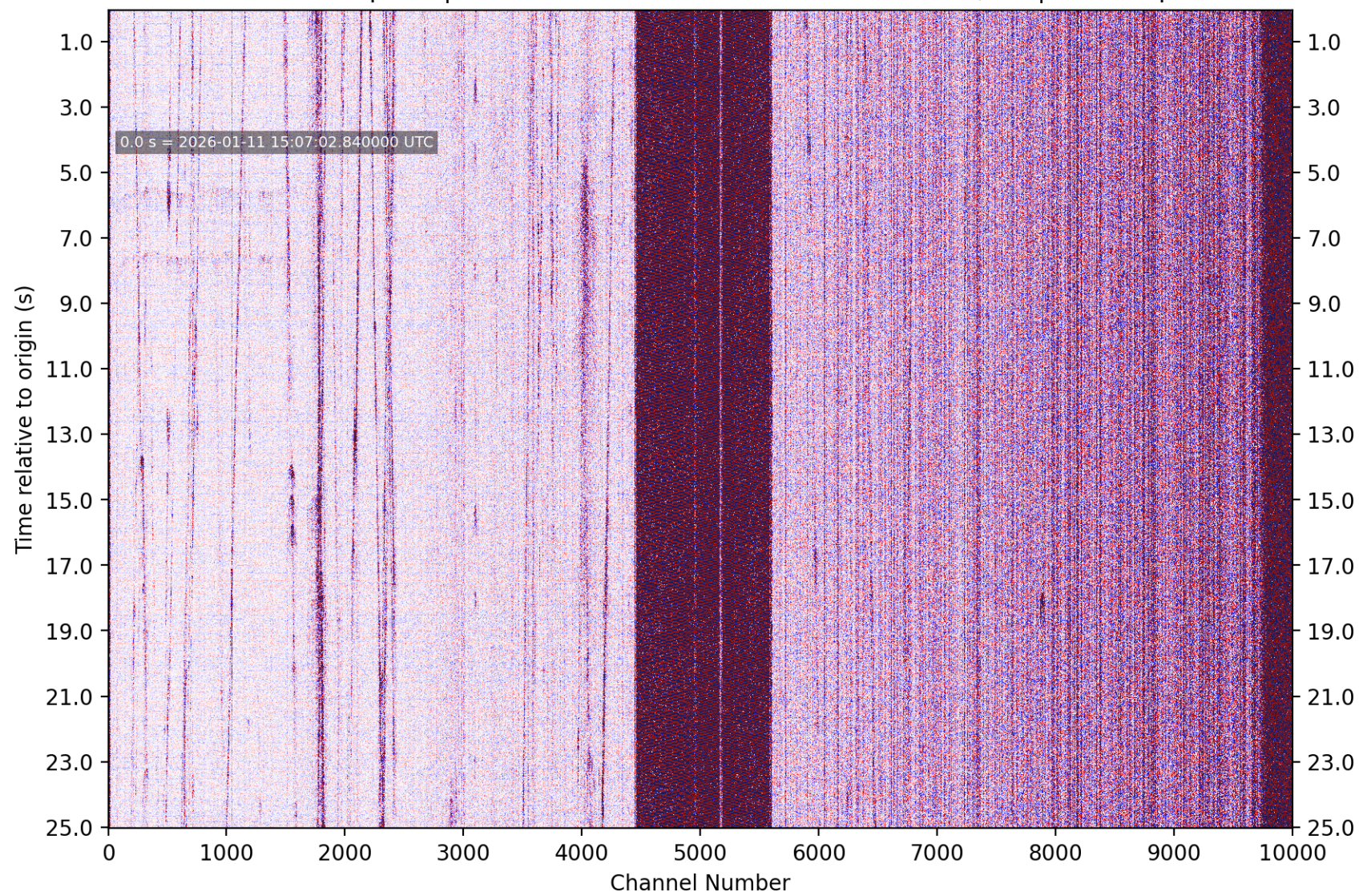
PhaseNet-DAS picks | nc75294121 M0.95 4 km SE of Pacifica, CA | without picks
