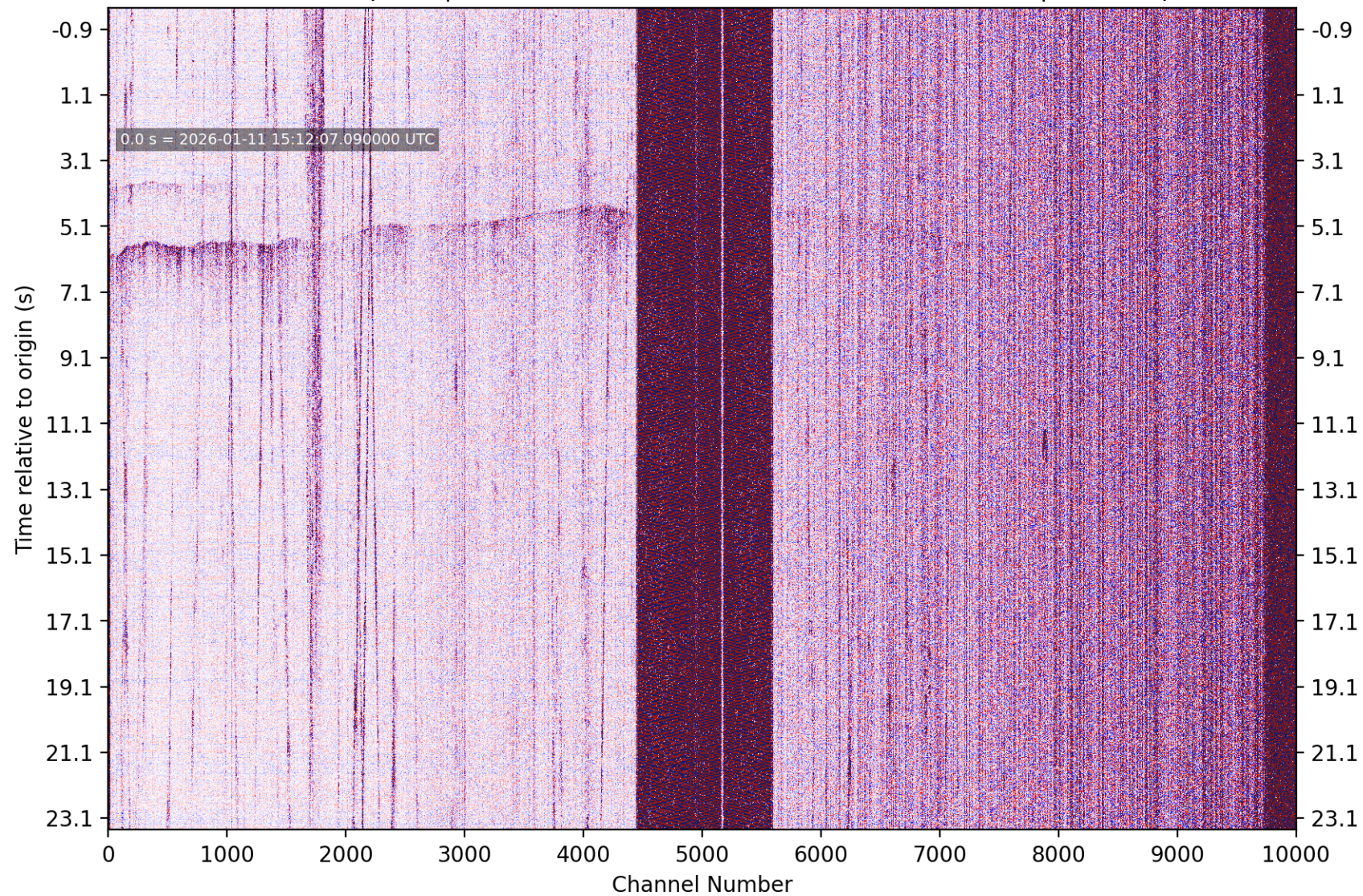
PhaseNet-DAS picks | nc75294126 M1.28 3 km SE of Pacifica, CA | without picks
