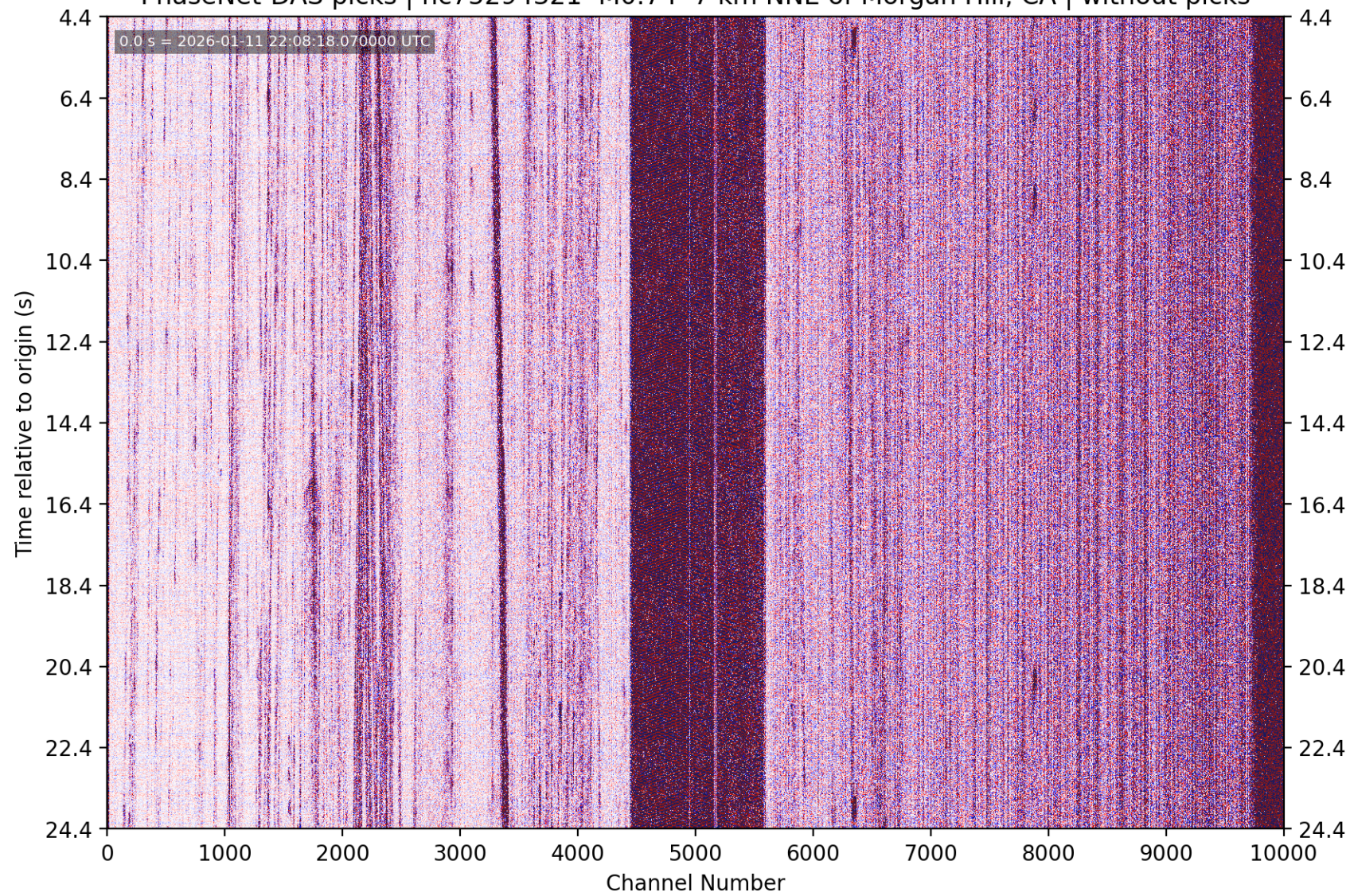
PhaseNet-DAS picks | nc75294321 M0.74 7 km NNE of Morgan Hill, CA | without picks
