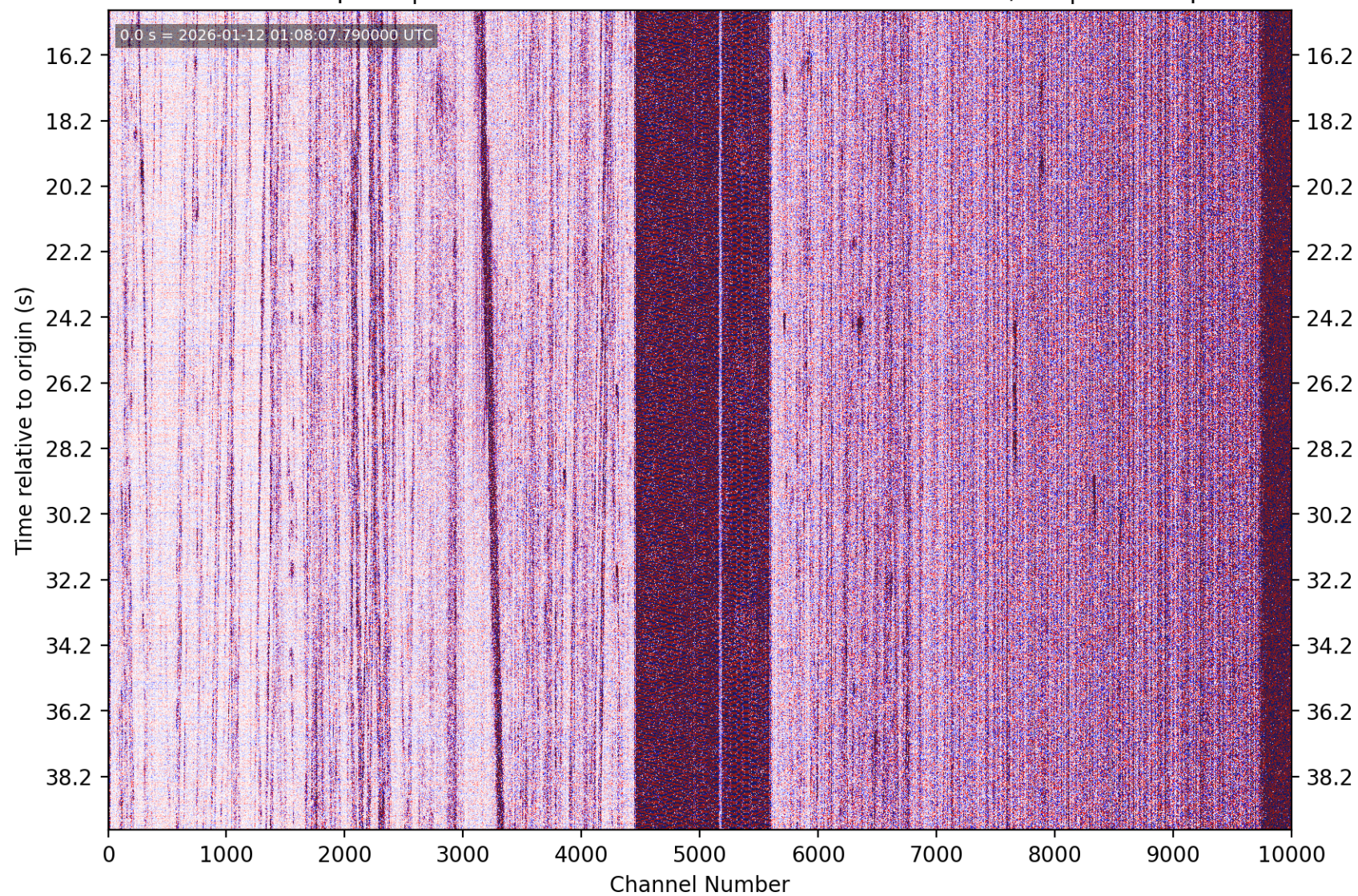
PhaseNet-DAS picks | nc75294401 M1.34 18 km SSE of Livermore, CA | without picks
