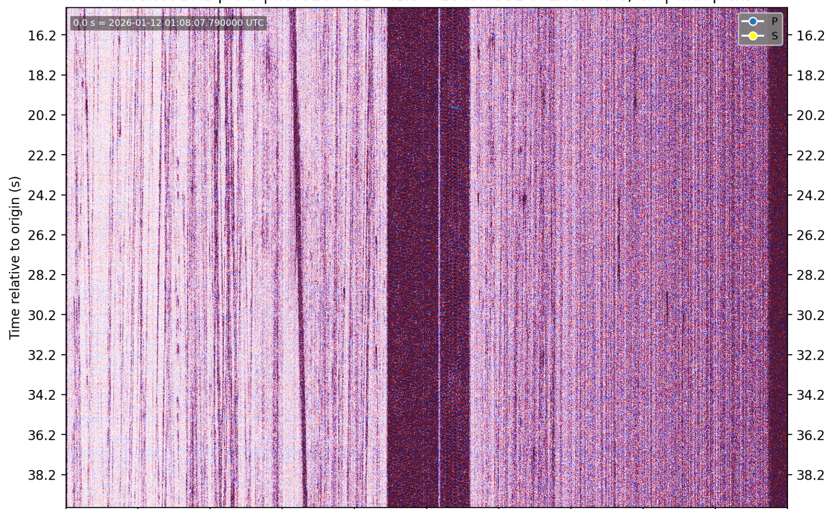
PhaseNet-DAS picks | nc75294401 M1.34 18 km SSE of Livermore, CA | without picks
