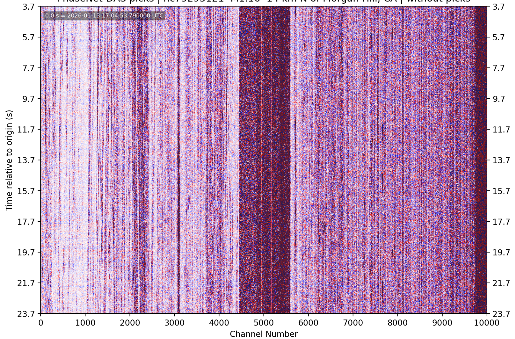
PhaseNet-DAS picks | nc75295121 M1.16 14 km N of Morgan Hill, CA | without picks
