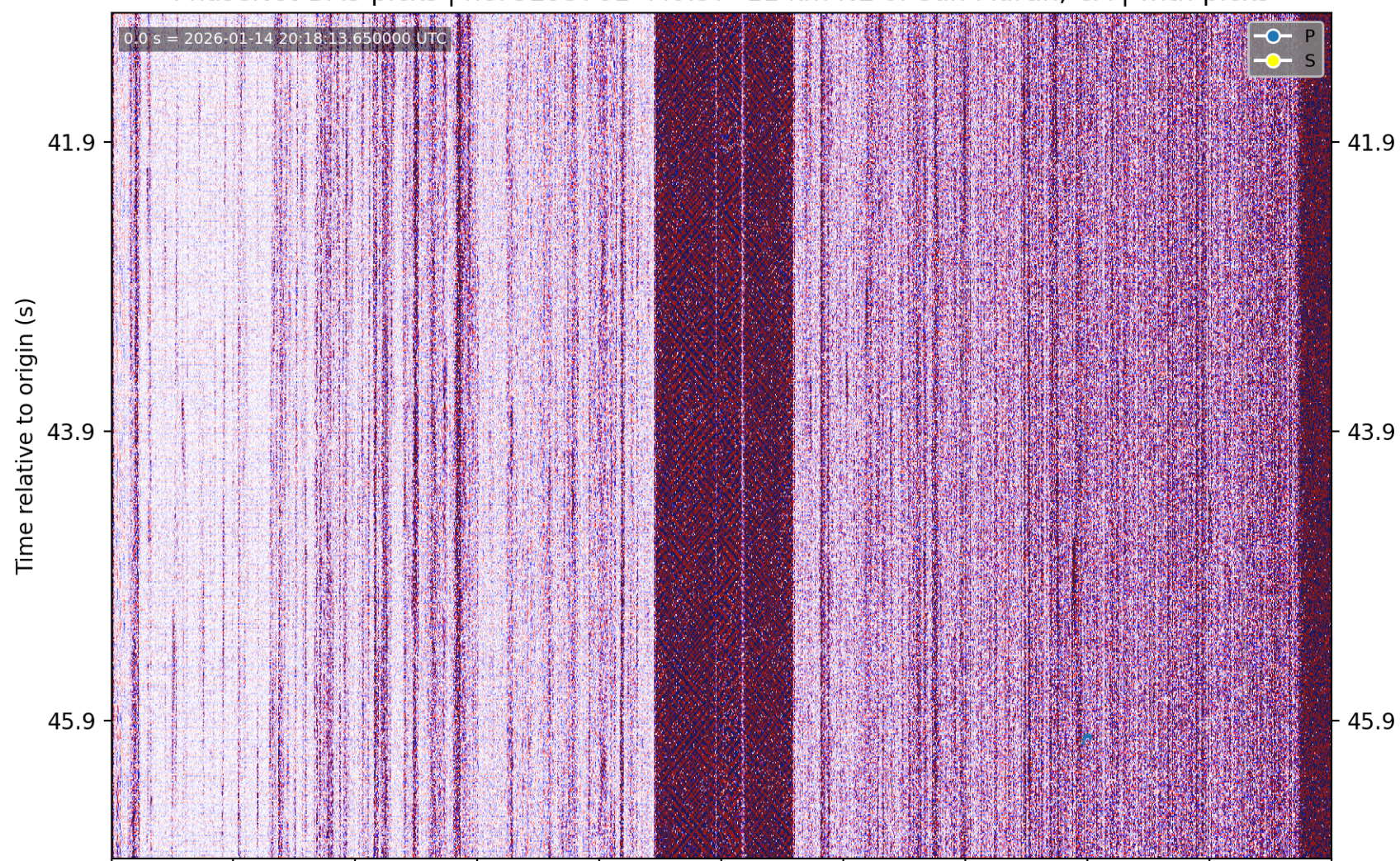
PhaseNet-DAS picks | nc75295781 M0.57 11 km NE of San Martin, CA | without picks
