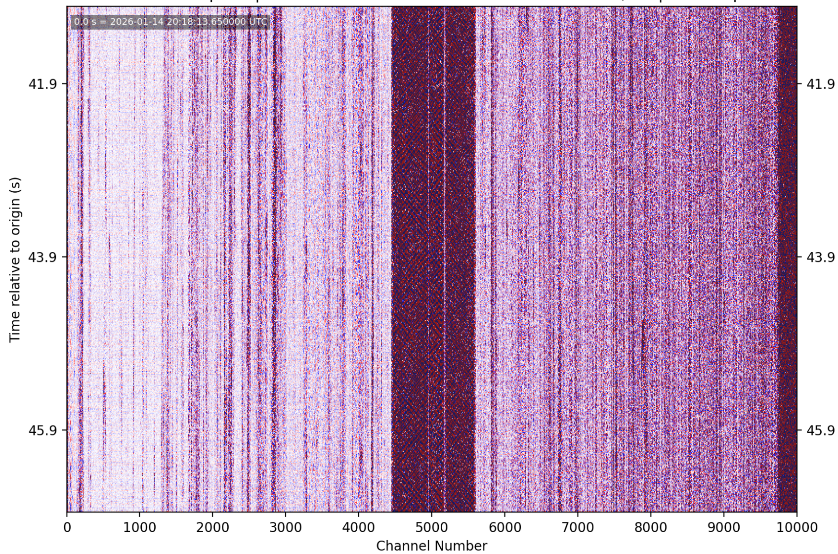
PhaseNet-DAS picks | nc75295781 M0.57 11 km NE of San Martin, CA | without picks
