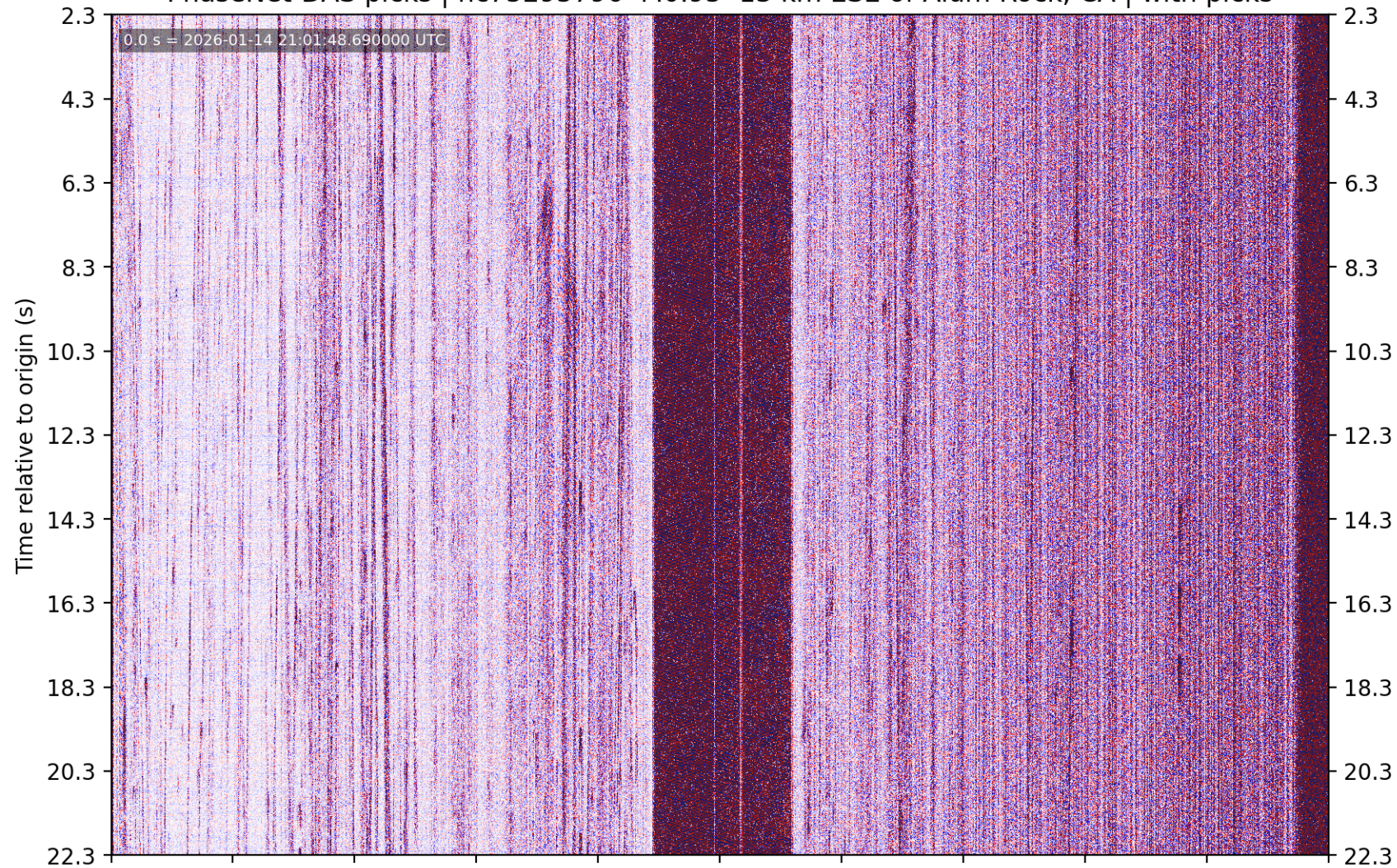
PhaseNet-DAS picks | nc75295796 M0.95 13 km ESE of Alum Rock, CA | without picks
