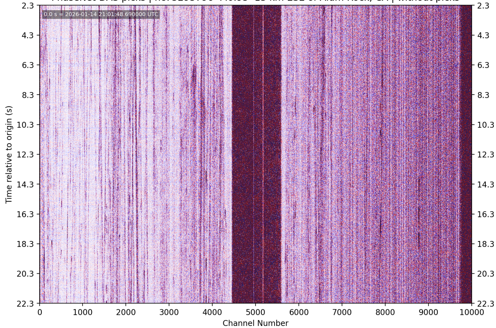
PhaseNet-DAS picks | nc75295796 M0.95 13 km ESE of Alum Rock, CA | without picks
