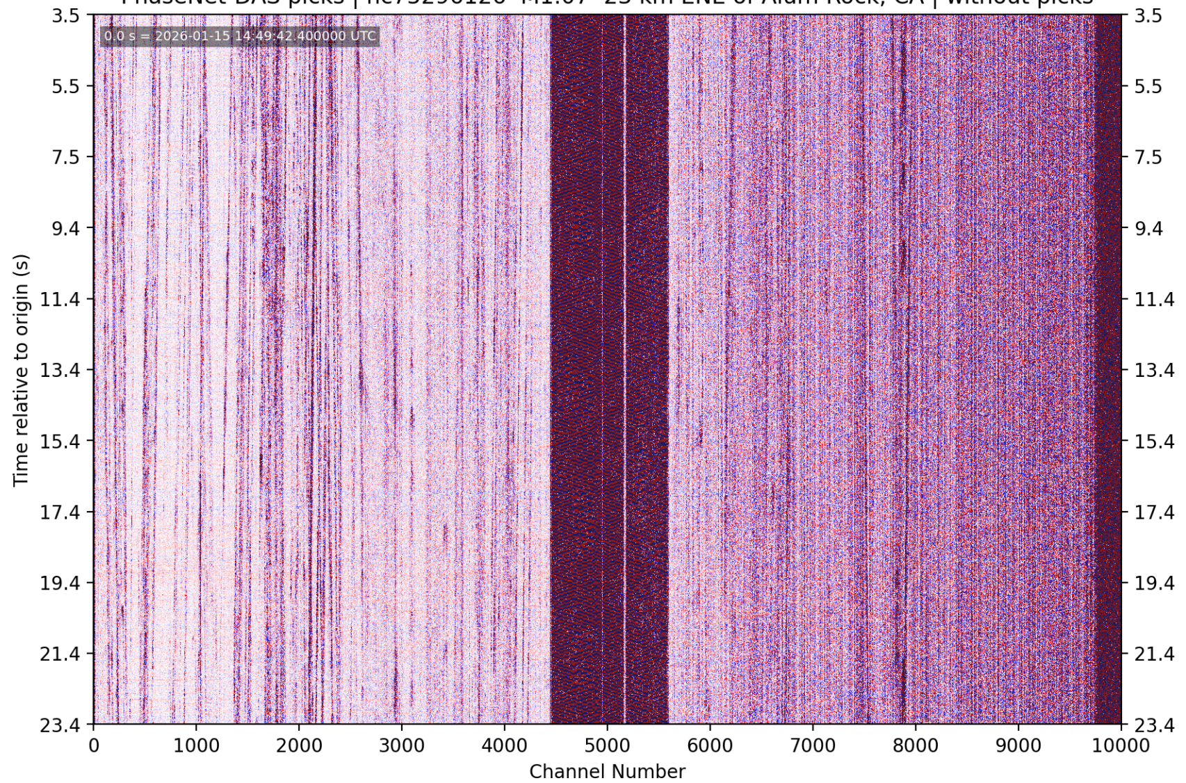
PhaseNet-DAS picks | nc75296126 M1.07 23 km ENE of Alum Rock, CA | without picks
