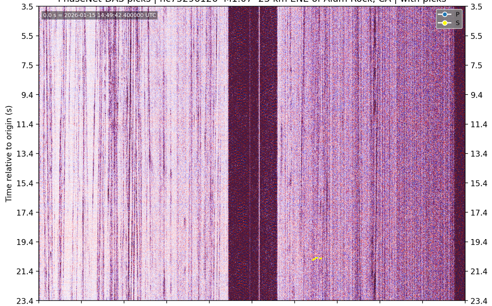
PhaseNet-DAS picks | nc75296126 M1.07 23 km ENE of Alum Rock, CA | without picks
