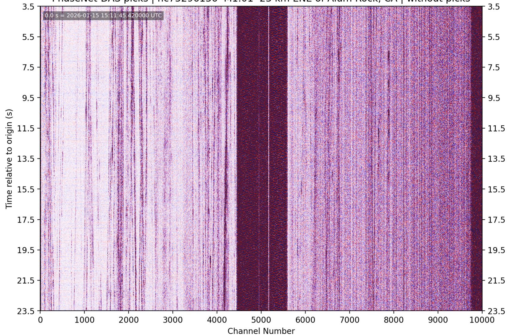
PhaseNet-DAS picks | nc75296136 M1.01 23 km ENE of Alum Rock, CA | without picks
