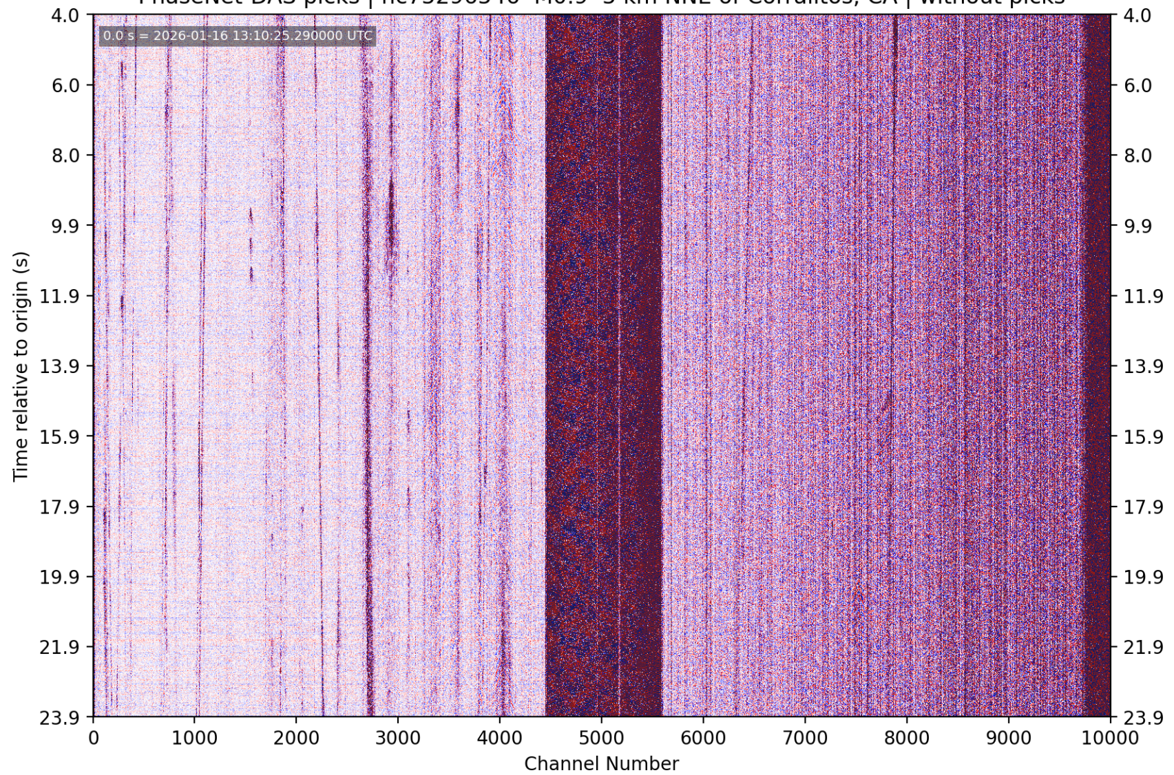
PhaseNet-DAS picks | nc75296546 M0.9 5 km NNE of Corralitos, CA | without picks
