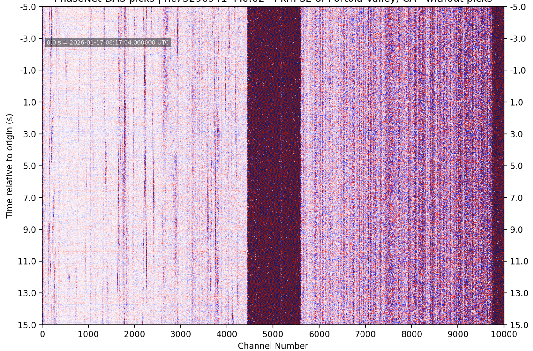
PhaseNet-DAS picks | nc75296941 M0.62 4 km SE of Portola Valley, CA | without picks
