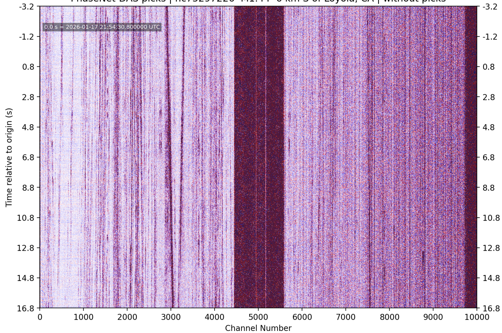
PhaseNet-DAS picks | nc75297226 M1.44 6 km S of Loyola, CA | without picks
