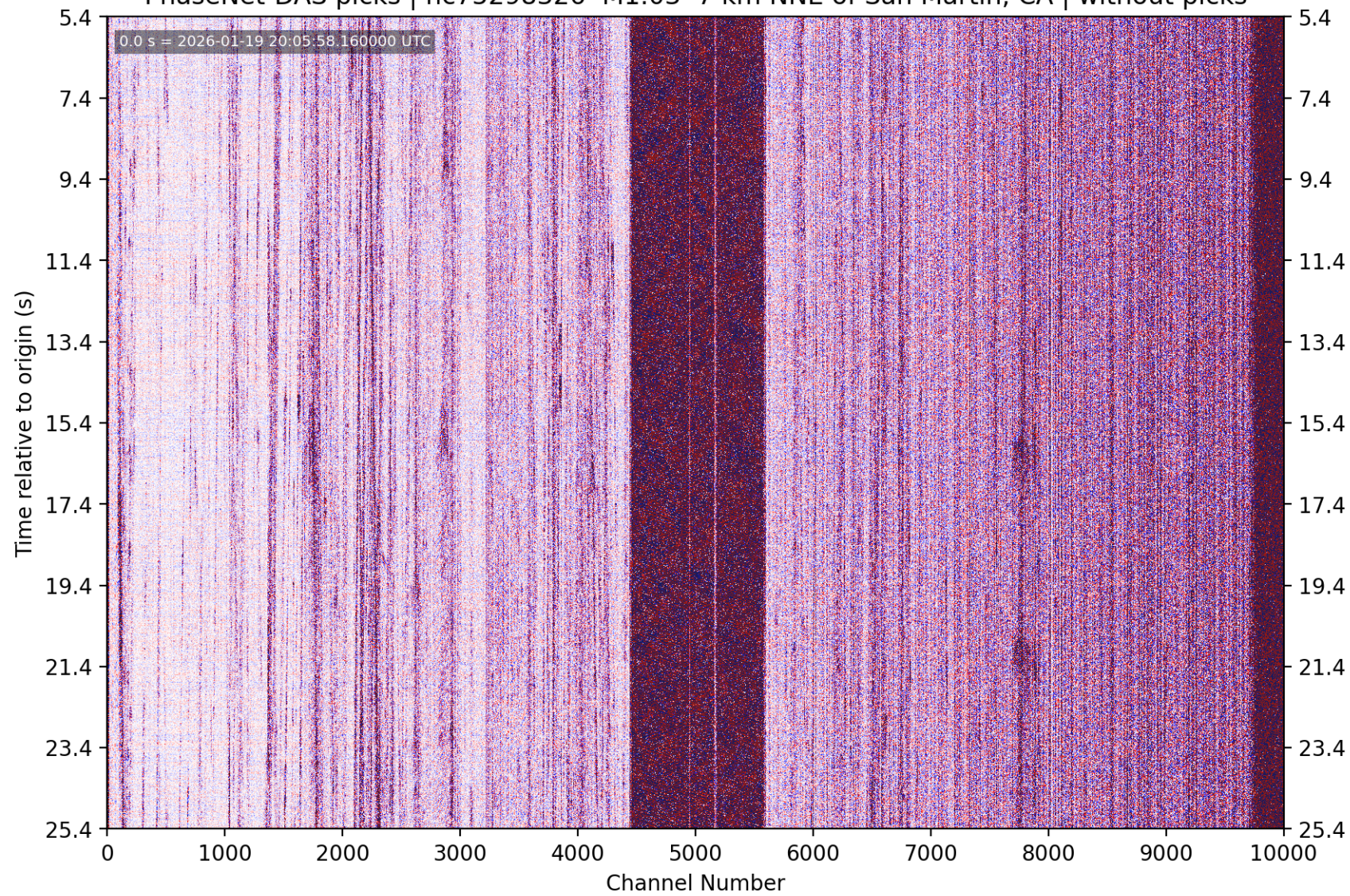
PhaseNet-DAS picks | nc75298326 M1.03 7 km NNE of San Martin, CA | without picks
