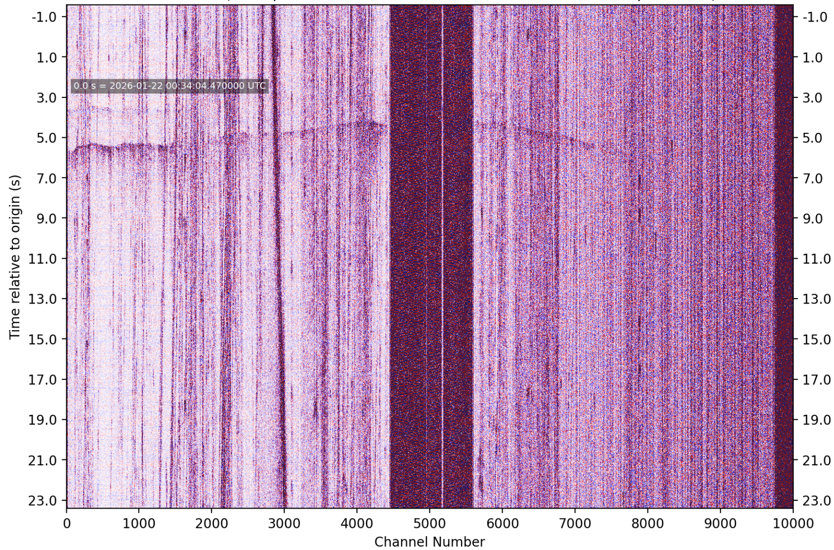
PhaseNet-DAS picks | nc75299596 M1.39 4 km SE of Pacifica, CA | without picks
