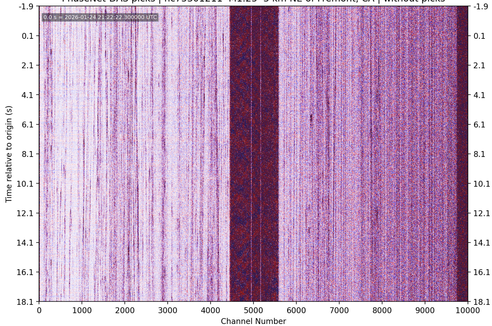
PhaseNet-DAS picks | nc75301211 M1.25 3 km NE of Fremont, CA | without picks
