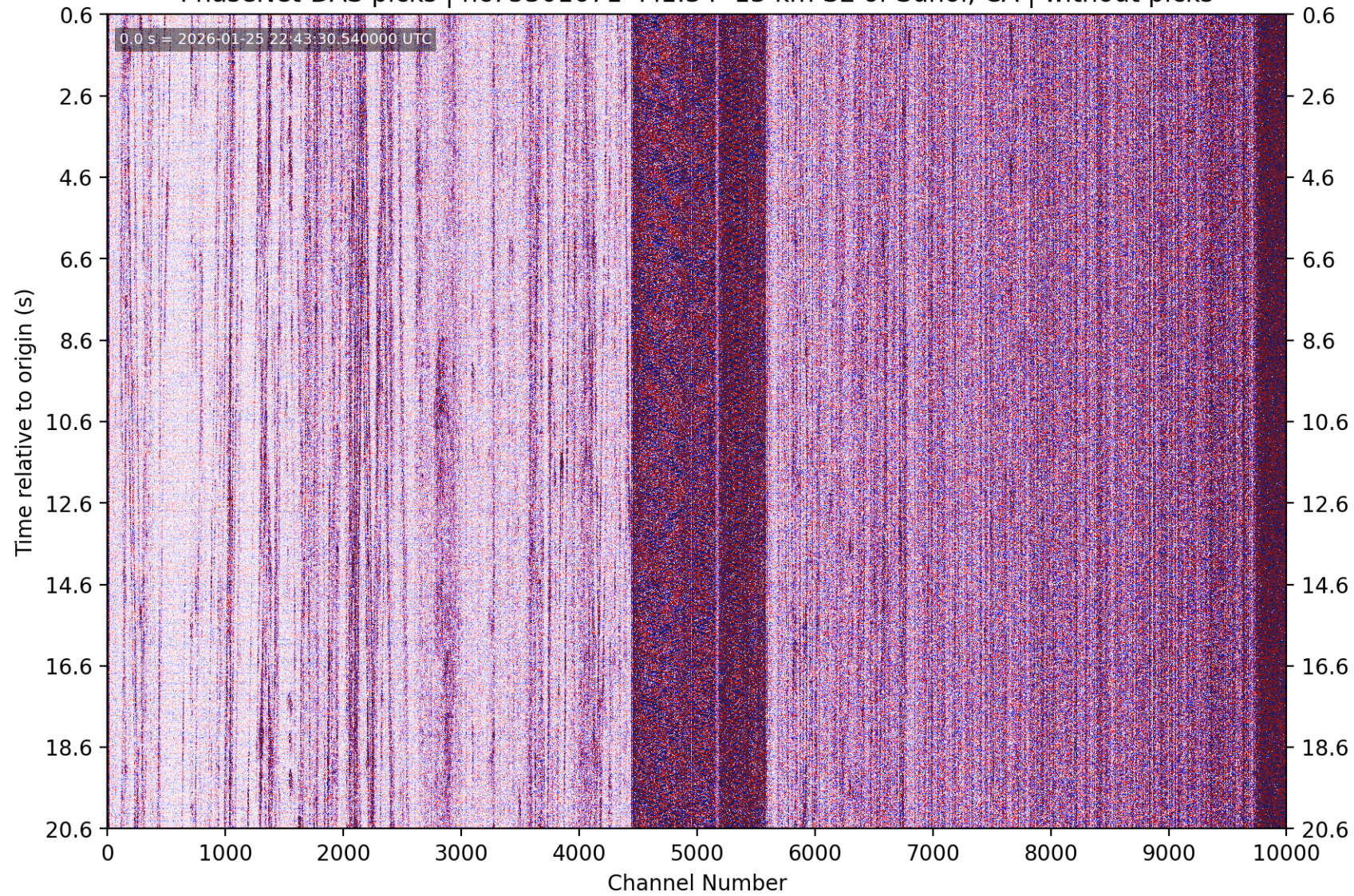
PhaseNet-DAS picks | nc75301671 M1.34 13 km SE of Sunol, CA | without picks
