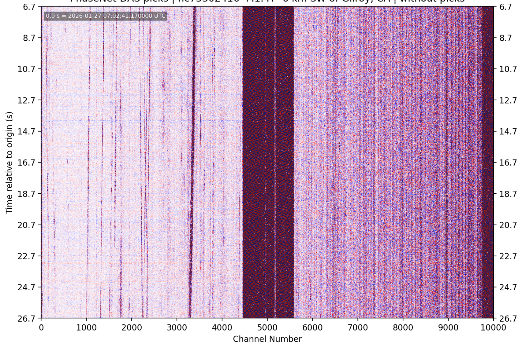
PhaseNet-DAS picks | nc75302416 M1.47 6 km SW of Gilroy, CA | without picks
