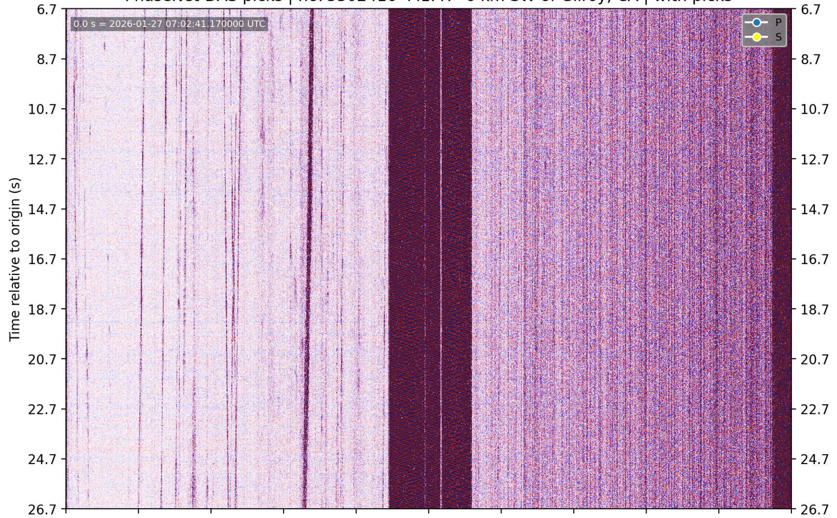
PhaseNet-DAS picks | nc75302416 M1.47 6 km SW of Gilroy, CA | without picks
