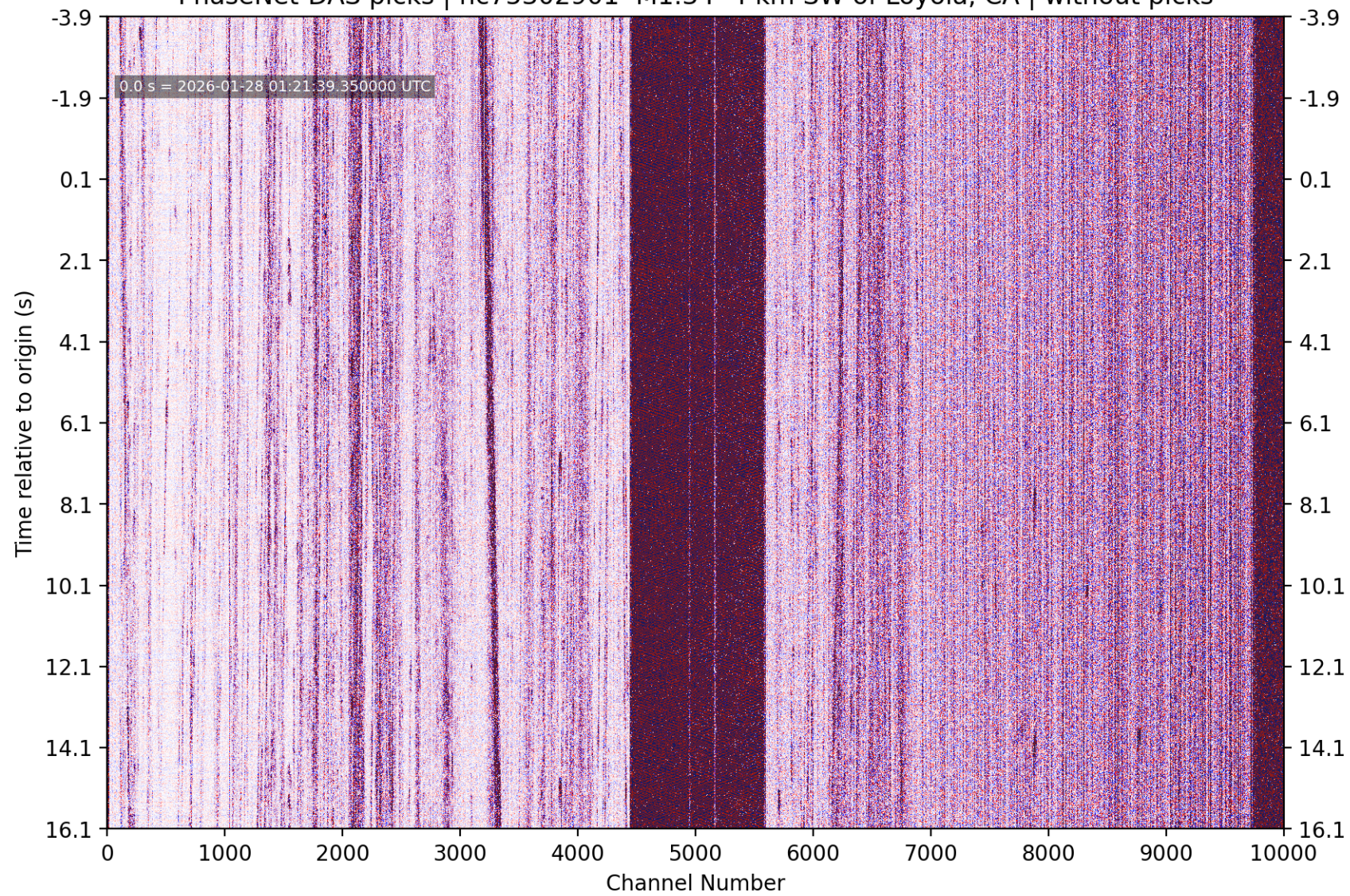
PhaseNet-DAS picks | nc75302901 M1.34 4 km SW of Loyola, CA | without picks
