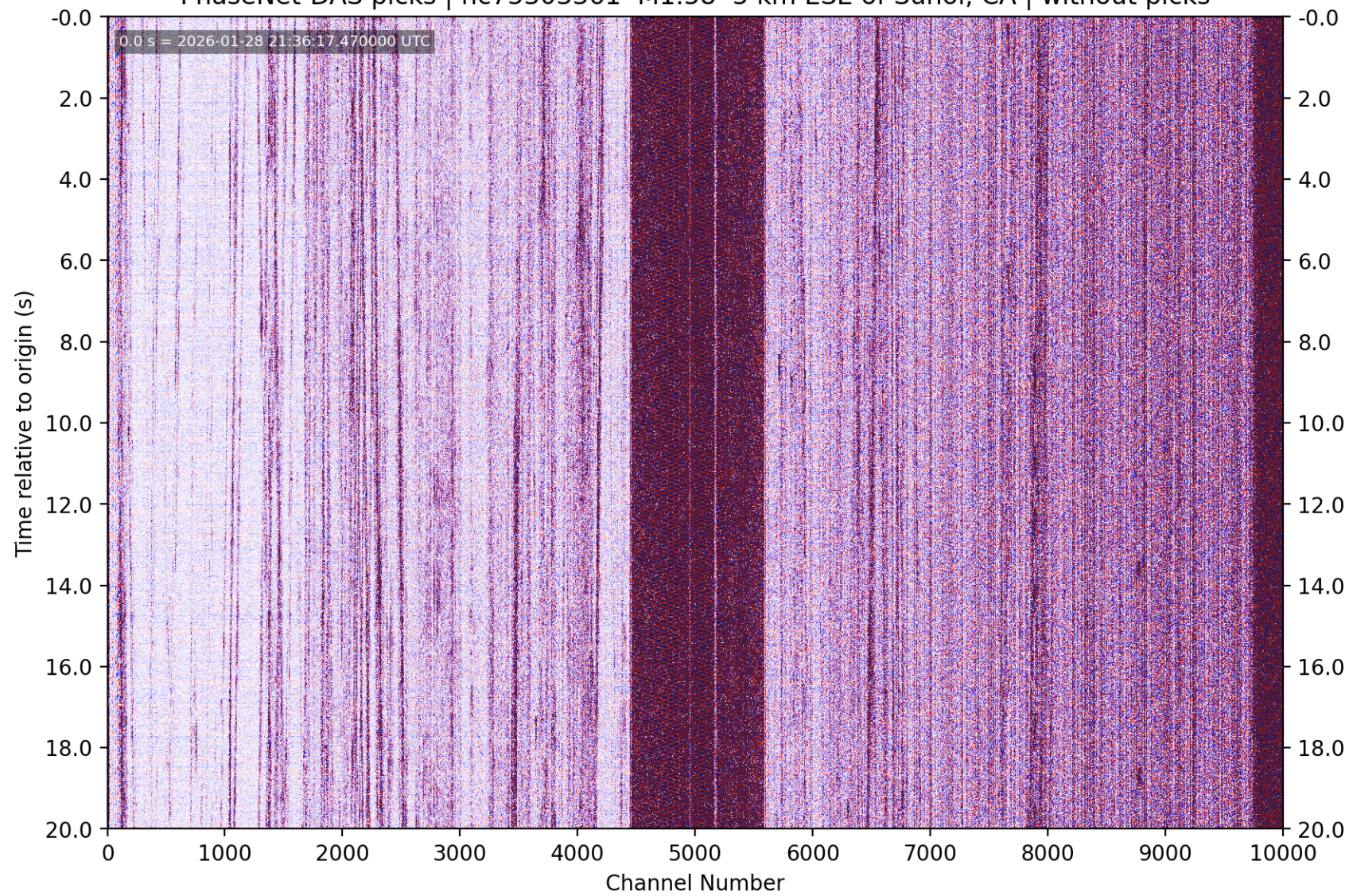
PhaseNet-DAS picks | nc75303361 M1.58 5 km ESE of Sunol, CA | without picks
